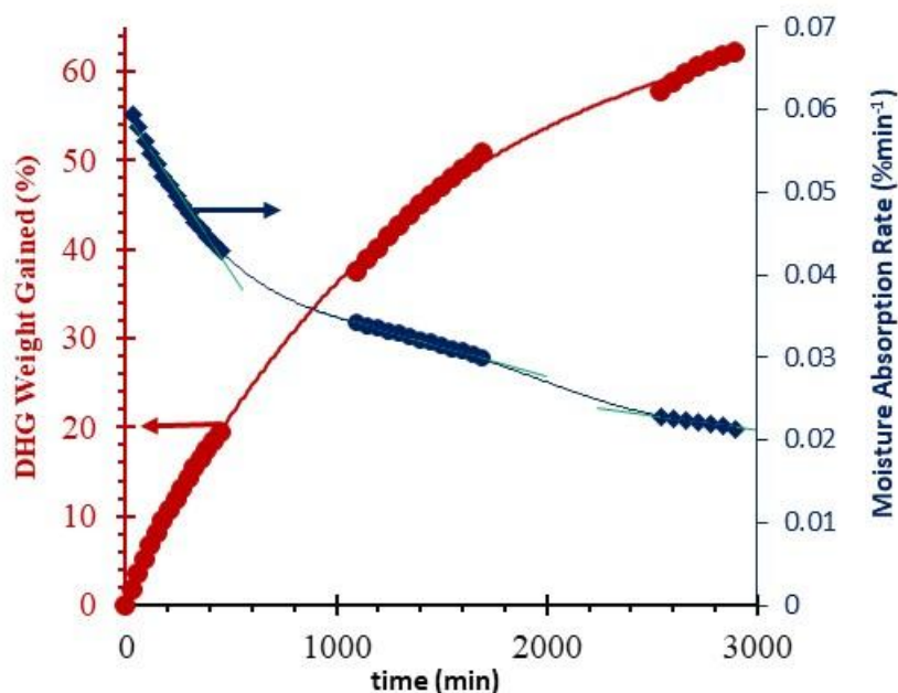
Fig. 1. DHG moisture absorption and its rate.
