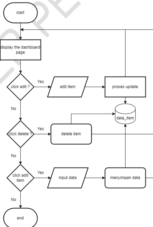
Figure 5 : Admin Page Flowchart
