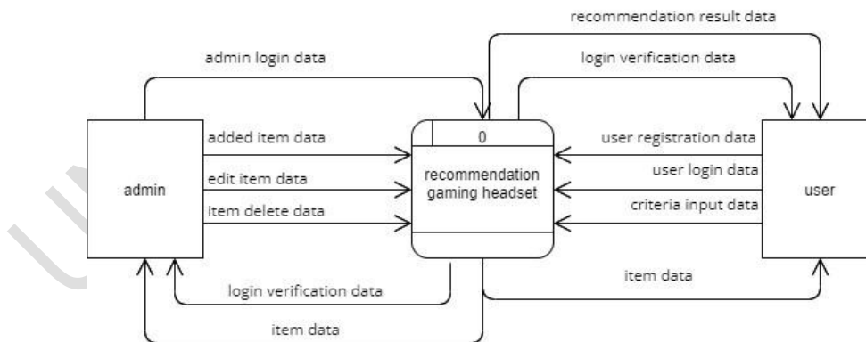
Figure 1 : DFD Level 0
