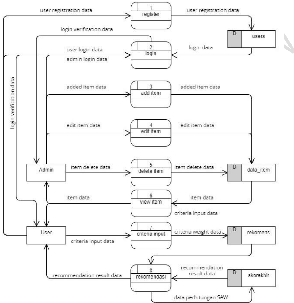
Figure 2 : DFD Level 1
