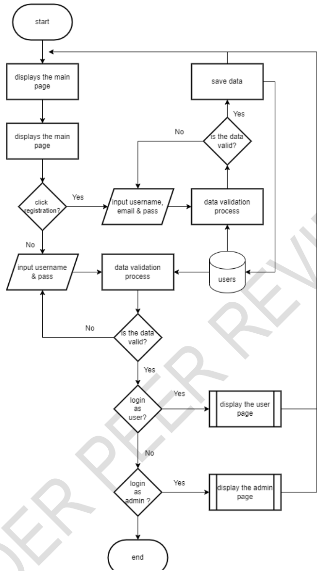
Figure 3 : Main Flowchart
