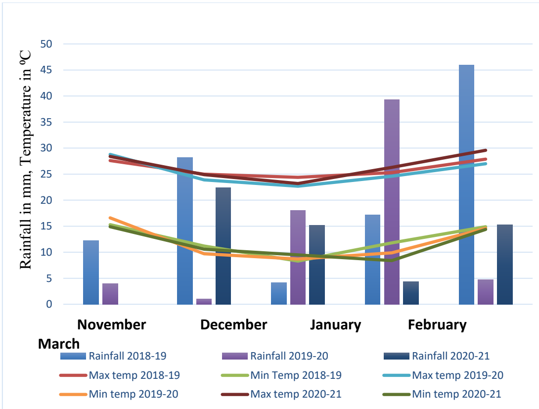
Fig 1: Weather parameters of three consecutive years during the crop season
