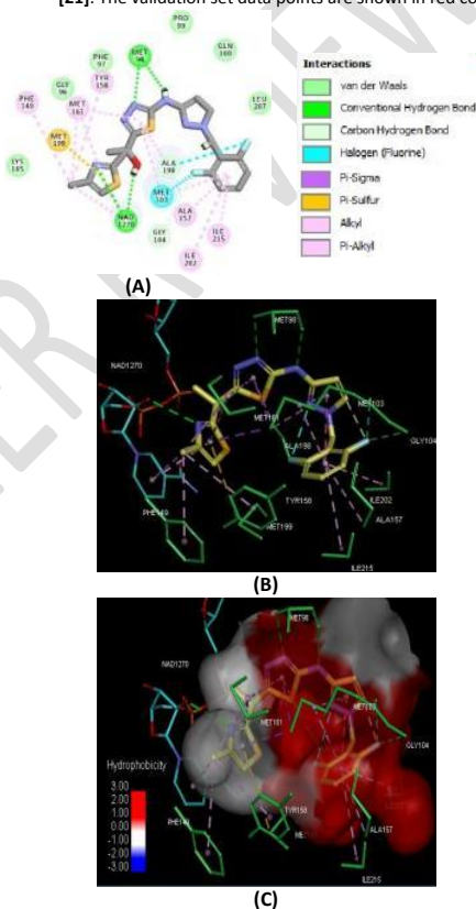
Figure 3: (A) 2D schematic interaction diagram of the most potent inhibitor TDZ1 ( IC_{50}^{exp} = 4 nM) [21] at the active site of InhA. (B) 3D structure of the active site of InhA with the most active inhibitor TDZ1. The carbon atoms of the ligand are colored in yellow, the residues' side chains in green, NAD cofactor carbon atoms are in cyan. Interaction color code: hydrogen bonds (green), Alkyl and Pi-Alkyl (pink), Pi-Sulfide (orange), Fluorine bond (blue). (C) Molecular surface of the active site of InhA. Surface coloring legend: red, hydrophobic; blue, hydrophilic; white, intermediate.
