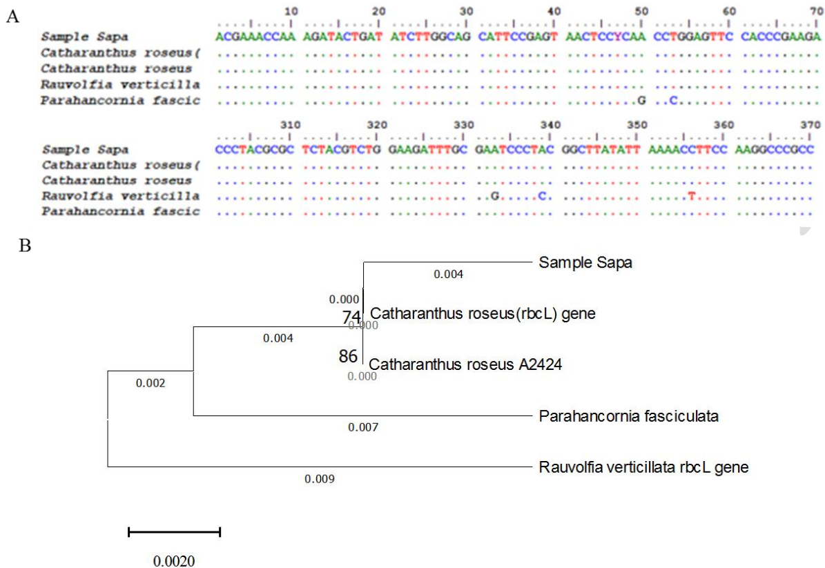
Figure 2. (A) Alignment of ribulose-1,5-bisphosphate carboxylase ( rbcL ) barcode region of five species. (B) The phylogenetic tree was constructed using the Neighbor-Joining method. The evolutionary distances were computed using the Kimura 2-parameter method and are in the units of the number of base substitutions per site. This analysis involved 5 nucleotide sequences. Evolutionary analyses were conducted in MEGA11.
