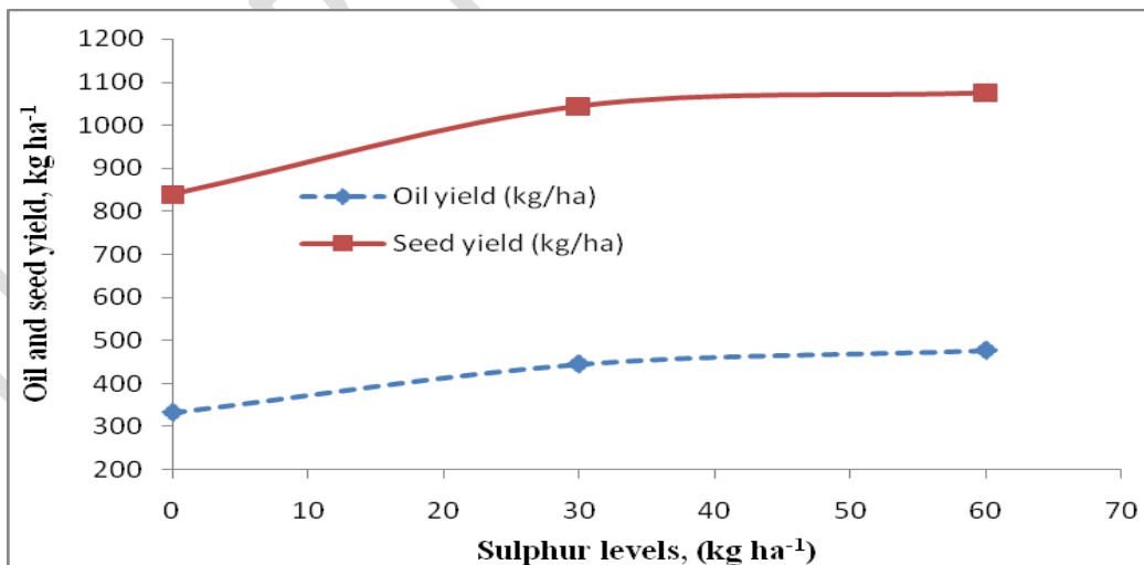
Fig. 3 Seed and oil yield of Indian mustard under different doses of Sulphur
