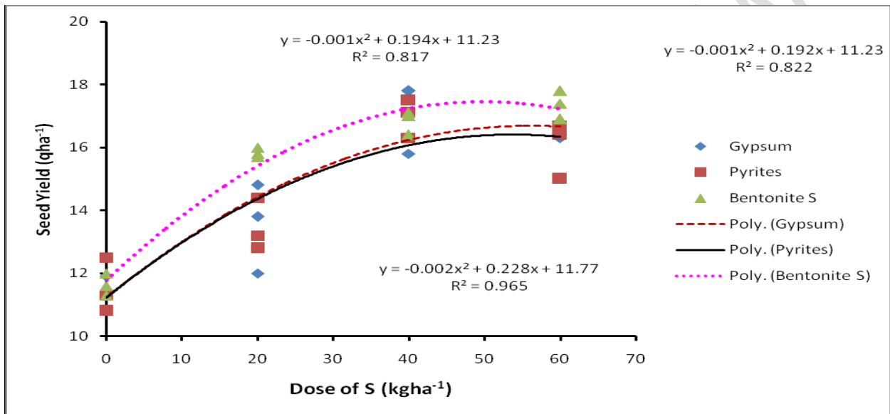
Figure 2 Yield response equation as influenced by sources and doses of sulphur
