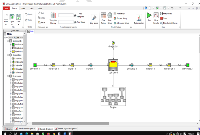
Plate 1: Engine Model from GT-POWER Software
