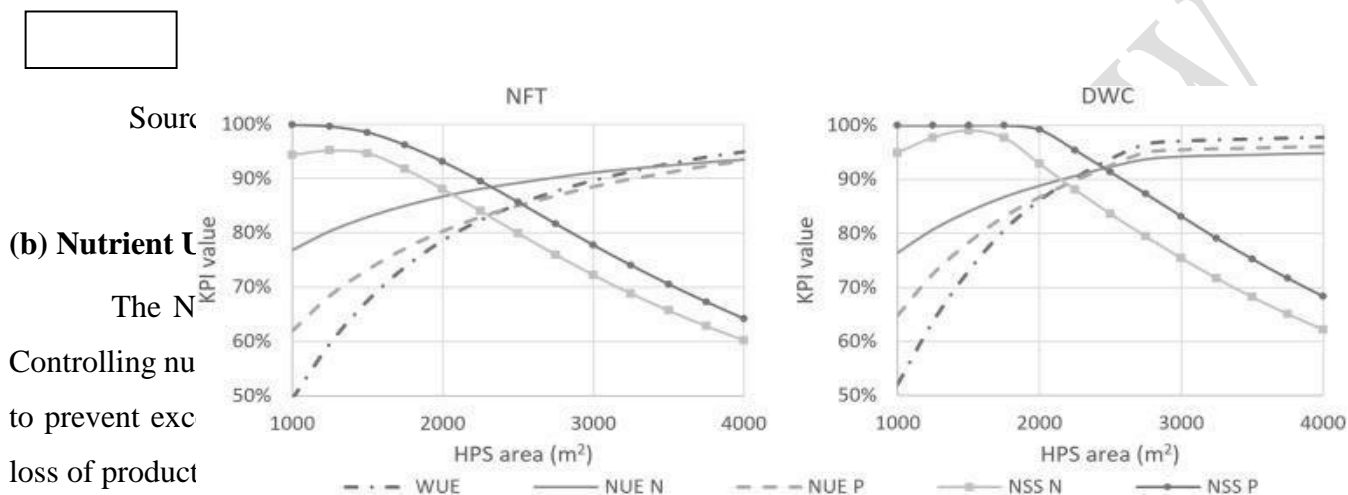
Fig 1. Shows the water and nutrient use efficiency of Nutrient Film Technology (NFT), & Deep Water Culture (DWC) System.
