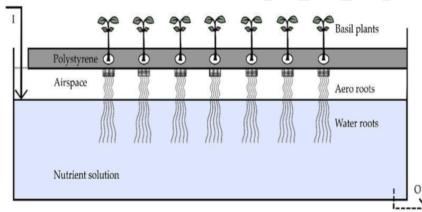
Fig 3. Dynamic Root Floating Technique.
