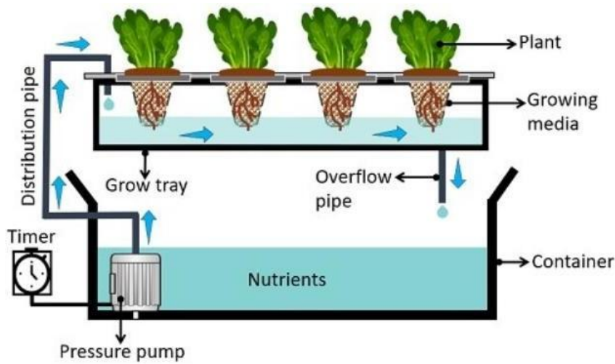
Fig 5. Ebb and Flow Method.
