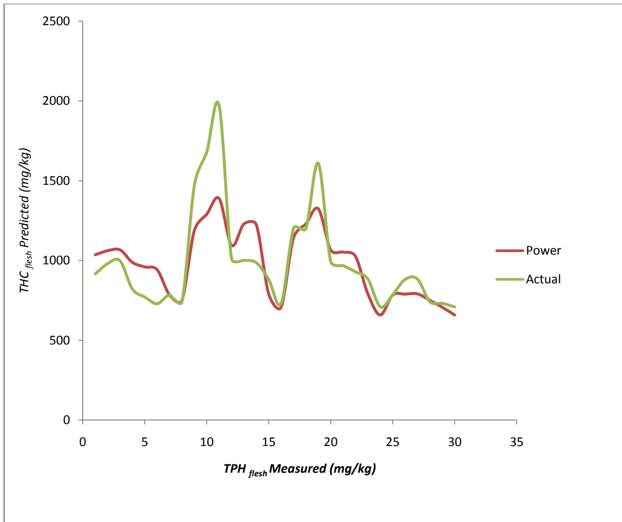
Figure 13: Graphical pattern of predicted THC flesh conc. in Tympanotomus fuscatus flesh against measured value
