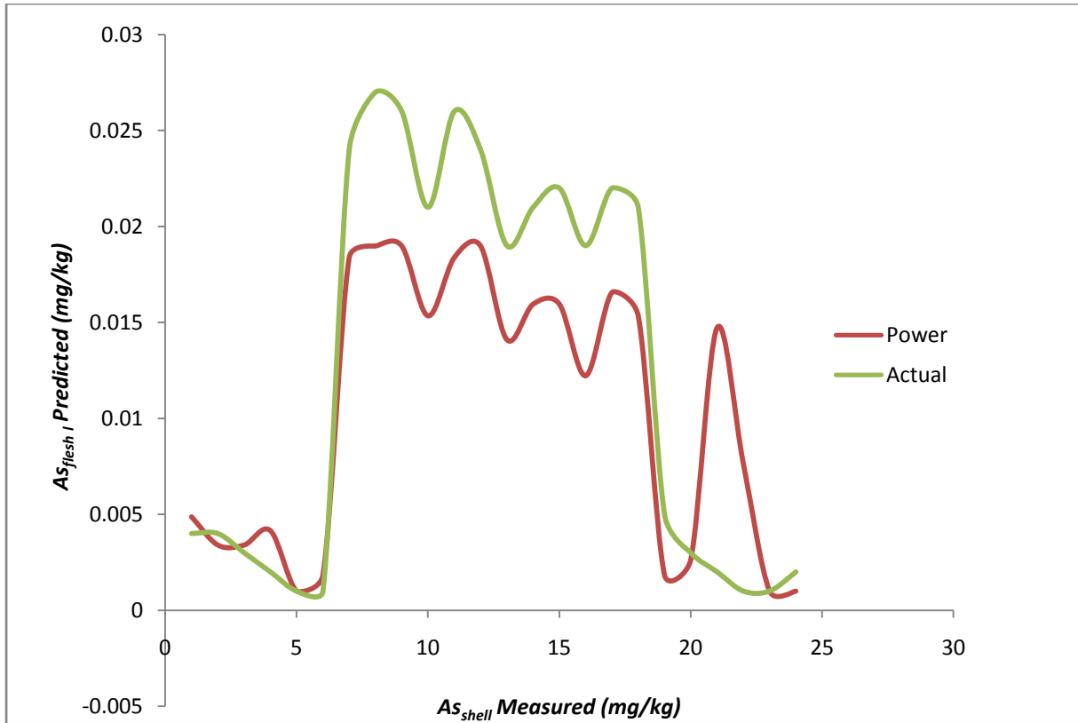
Figure 3: Graphical pattern of predicted As conc. in Ostreidae flesh against measured value
