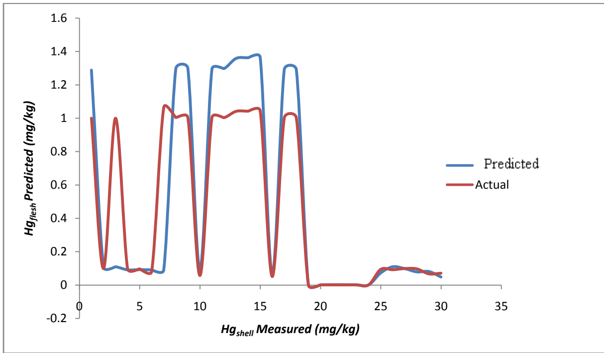
Figure 5: Graphical pattern of predicted Hg conc. in Ostreidae flesh against measured value
