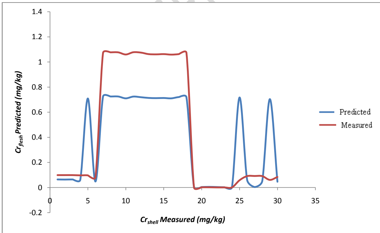
Figure 4: Graphical pattern of predicted Cr conc. in Ostreidae flesh against measured value
