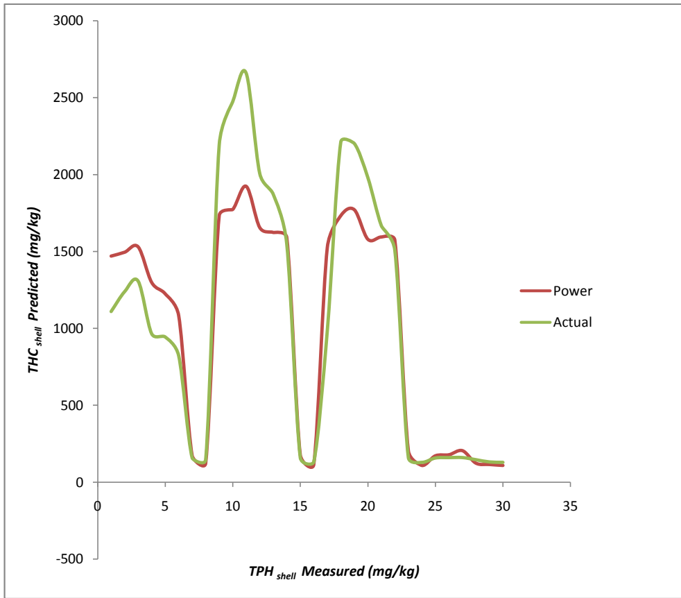
Figure 12: Graphical pattern of predicted THC shell conc. in Tympnotomus fuscatus flesh against measured value
