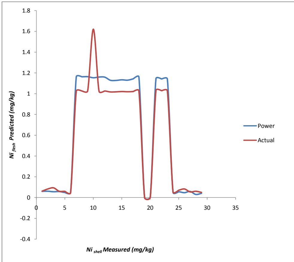
Figure 11: Graphical pattern of predicted Ni conc. in Tympanotomus fuscatus flesh against measured value
