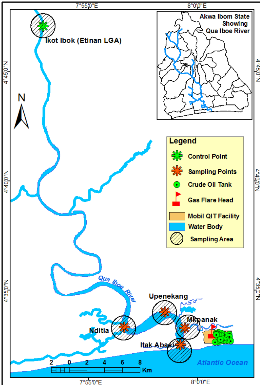
Fig 1: Location of Sampling Points along Qua-Iboe River
