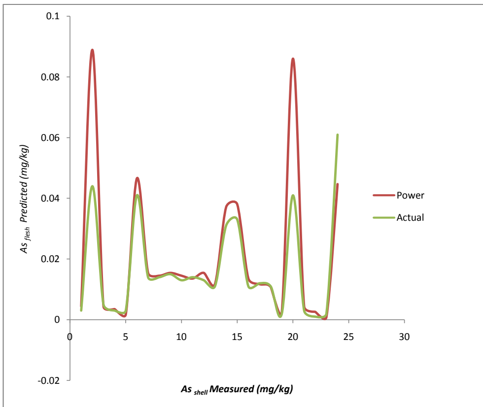
Figure 10: Graphical pattern of predicted As conc. in Typanotomus fuscatus flesh against measured value
