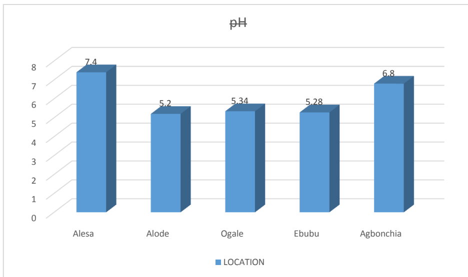
Fig. 5: Graphical presentation of pH in the water samples Location
