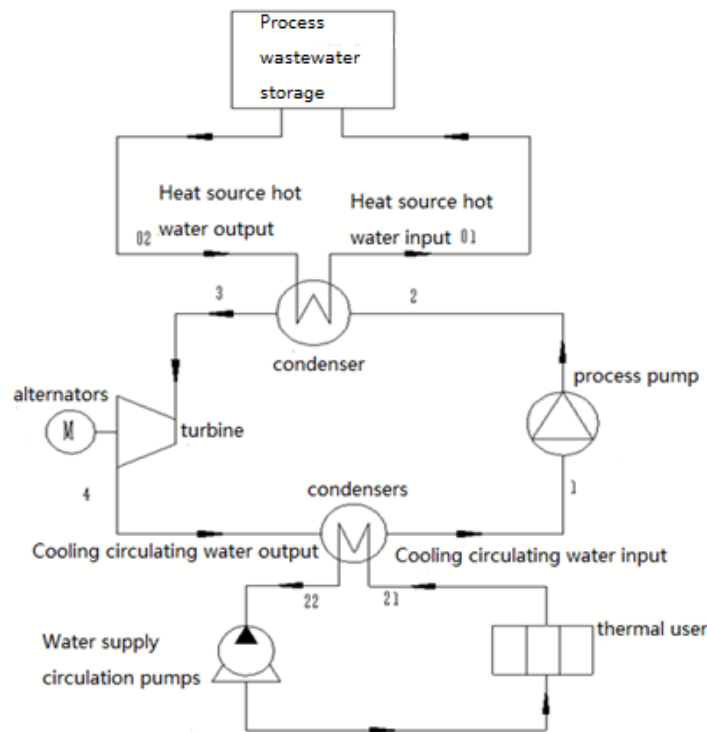
Figure 1 Schematic diagram of cogeneration system
