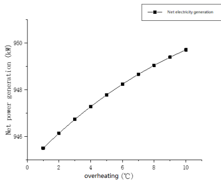
c overheating
