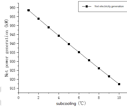
d subcooling
