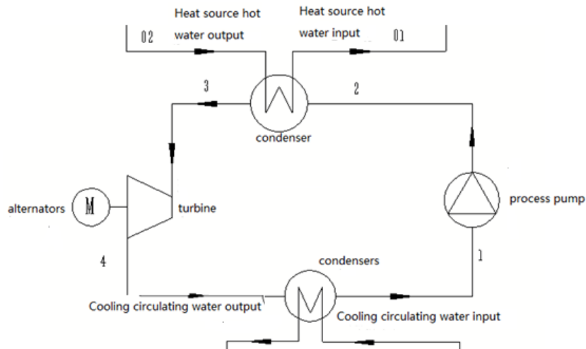
Figure 4 ORC Power Generation System Flowchart
