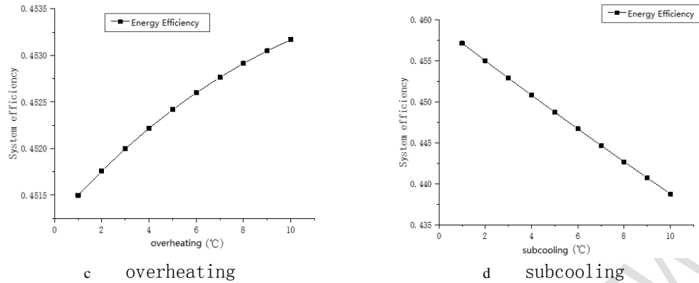
Figure 6 Impact of variable factors on energy efficiency
