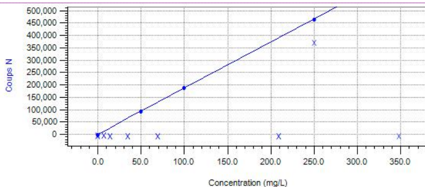
Figure 1: Calibration curve
