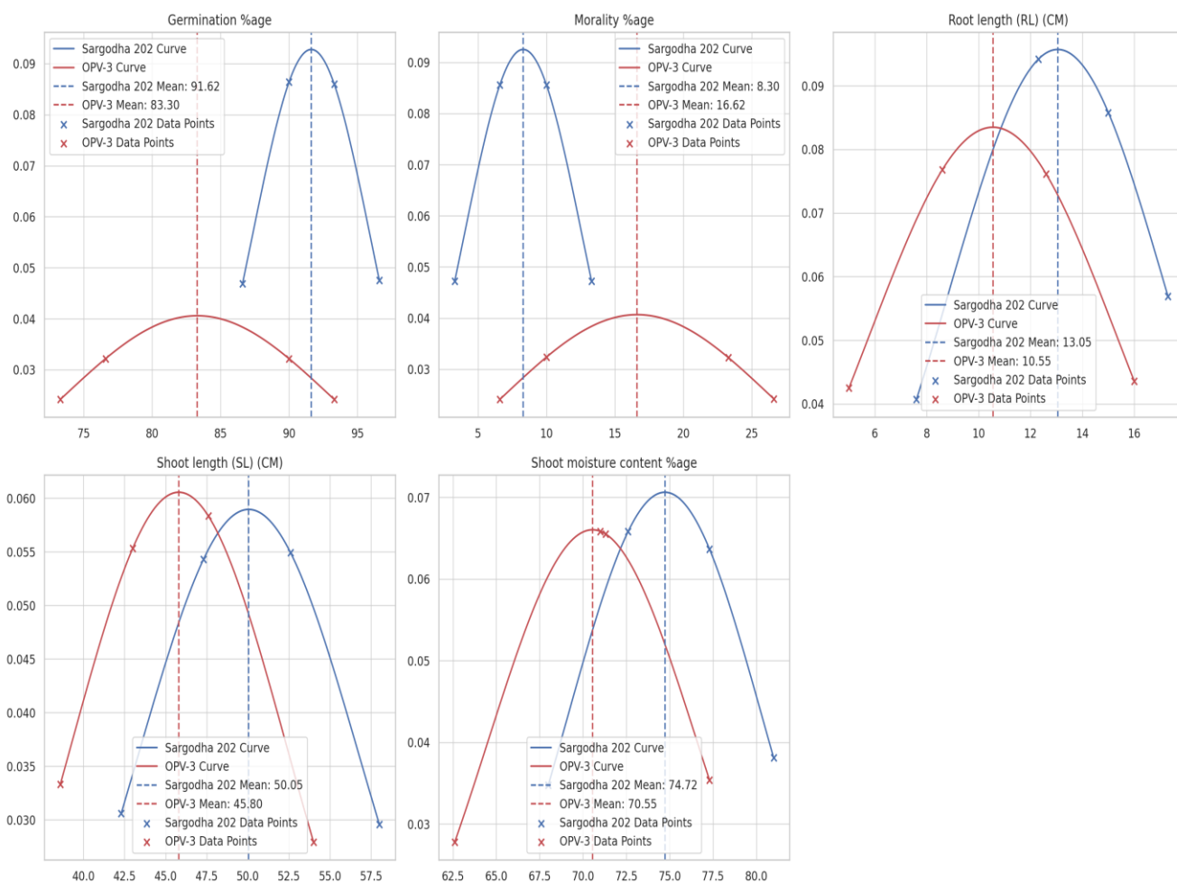
Distribution of Parameters for Sargodha 202 and OPV-3 with Mean Lines and Data Points
