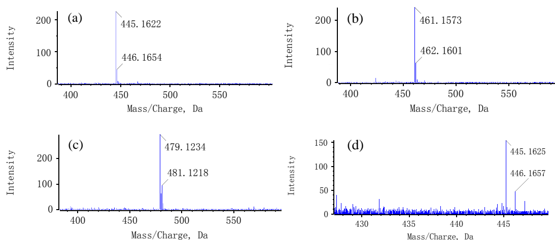
Fig. 4. The high resolution mass spectra of (a)TC, (b)oxytetracycline , (c)chlortetracycline, and (d)doxycycline
