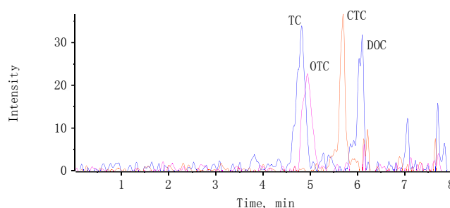
Fig. 5. The chromatogram of four tetracyclines at LOD concentration level
