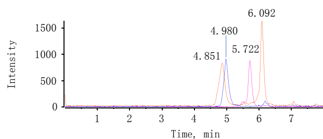
Fig. 3. Optimized chromatogram of TC (4.85 min), oxytetracycline(4.98 min), chlortetracycline (5.72 min), and doxycycline (6.09 min) under gradient program.
