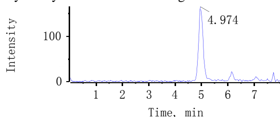
Fig. 7. Chromatogram (SIC) of oxytetracycline detected in the wastewater sample.
