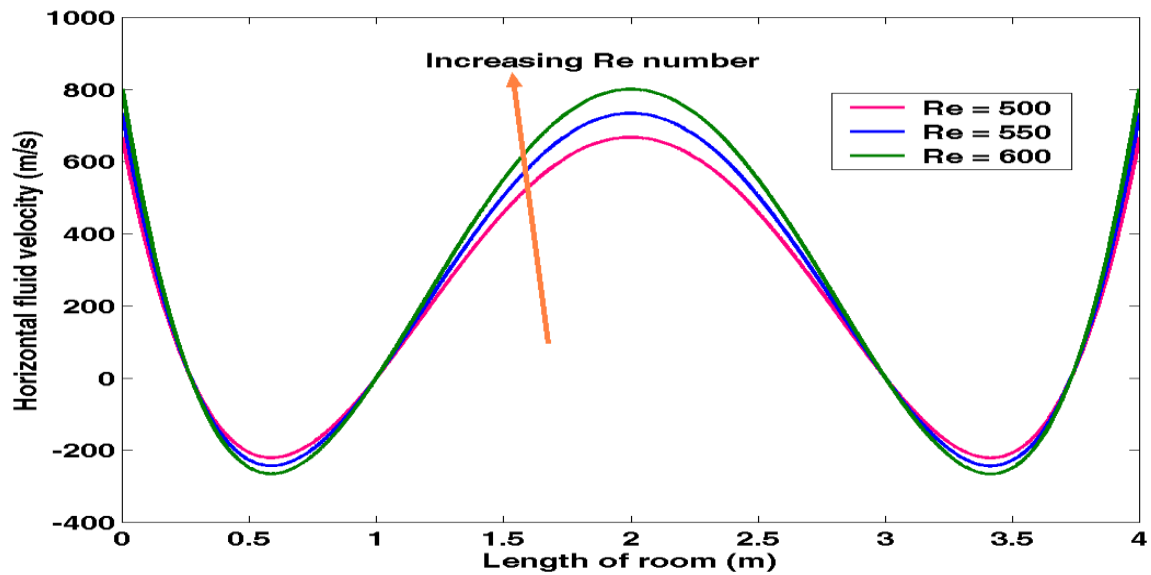
Figure 1: A graph of horizontal velocity against Length of room at varying Reynolds' number
