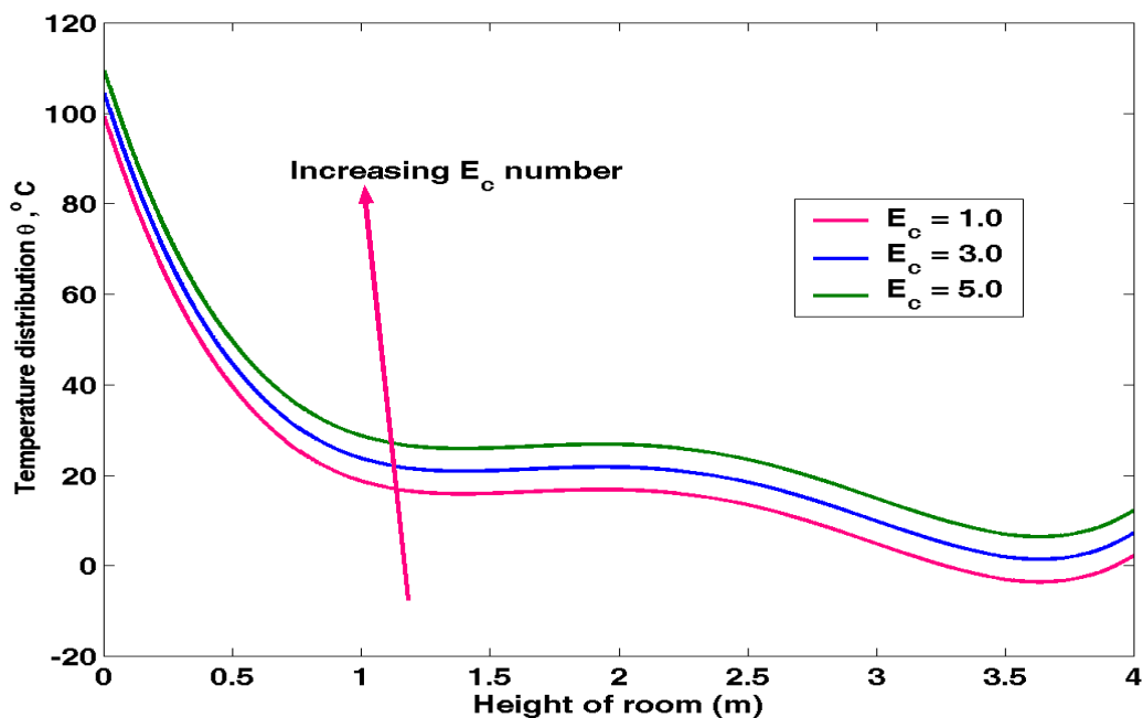
Figure 4: A graph of temperature distribution against Room Height at varying Eckert number
