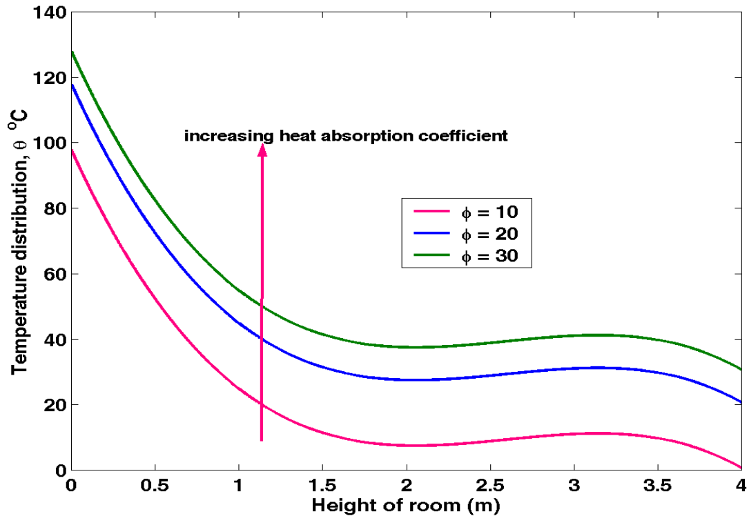
Figure 5: A graph of temperature distribution against room Height at varying heat absorption coefficient
