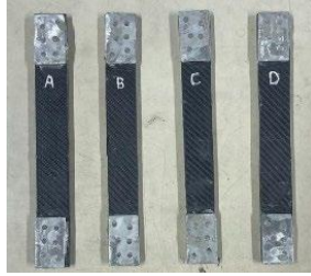
Fig. 10 Bio-composite tensile test specimens
