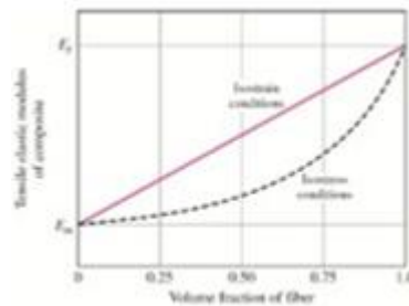
Fig. 6 Comparison of composite iso-strain and iso-stress conditions
