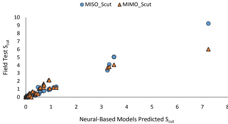
Figure 12: Generalization Performance of MISO and MIMO models predicted S_{cut} with field test datasets
