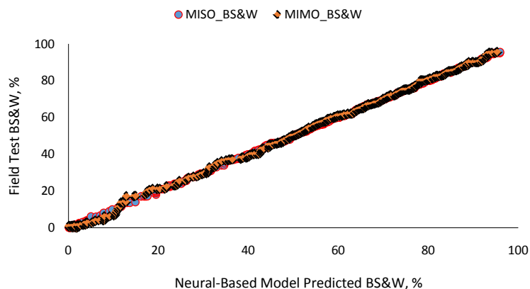
Figure 9: Comparison of MISO and MIMO predicted BS&W with field datasets
