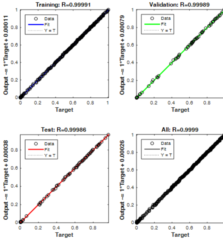
Figure 4: Regression plot of the BS&W network training, validation, and testing performance
