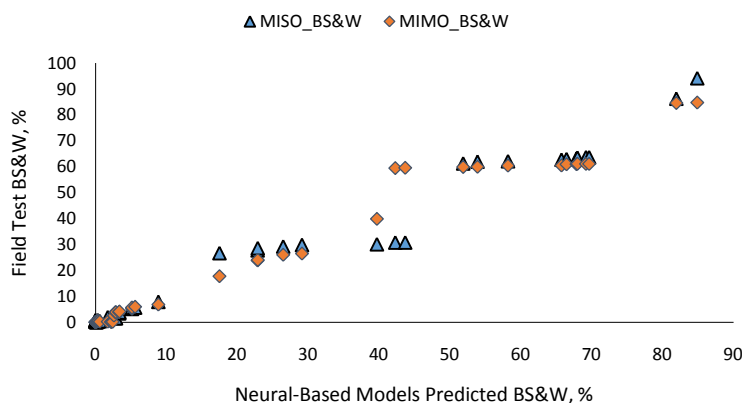
Figure 11: Generalization Performance of MISO and MIMO models BS&W with field test datasets
