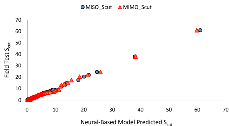
Figure 10: Comparison of MISO and MIMO predicted S_{cut} with field datasets
