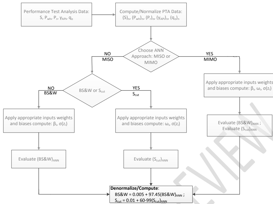
Figure 13: Software application flowchart of the developed neural-based models
