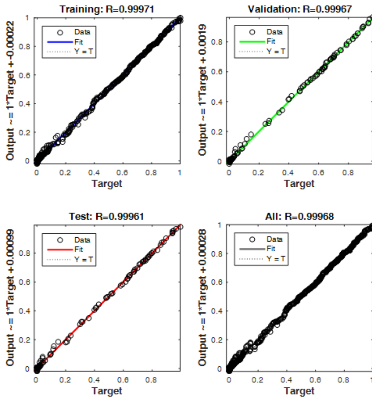
Figure 8: Regression plot of the S_{cut} network training, validation and testing performance
