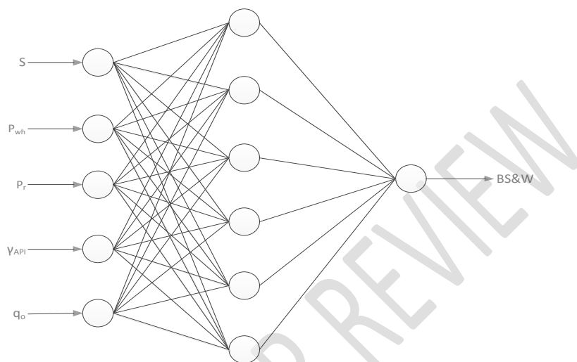
Figure 3: ANN Topology for BS&W Model
