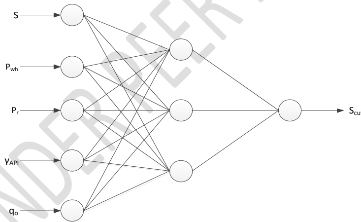
Figure 5: ANN Topology for S_{cut} Model
