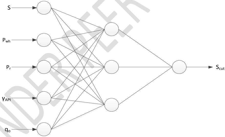
Figure 5: ANN Topology for S_{cut} Model
