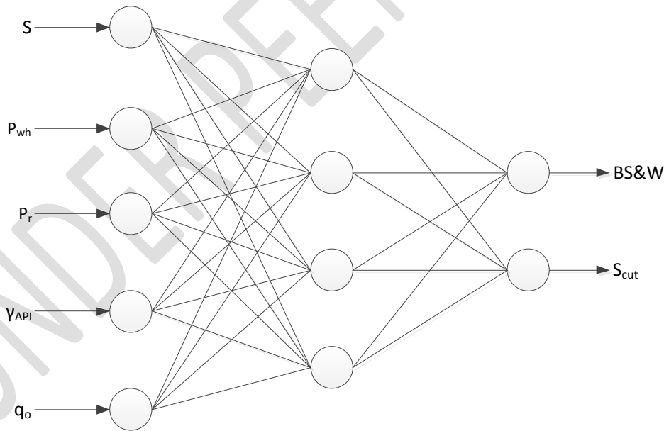
Figure 7: ANN Topology for BS&W- S_{cut} Model
