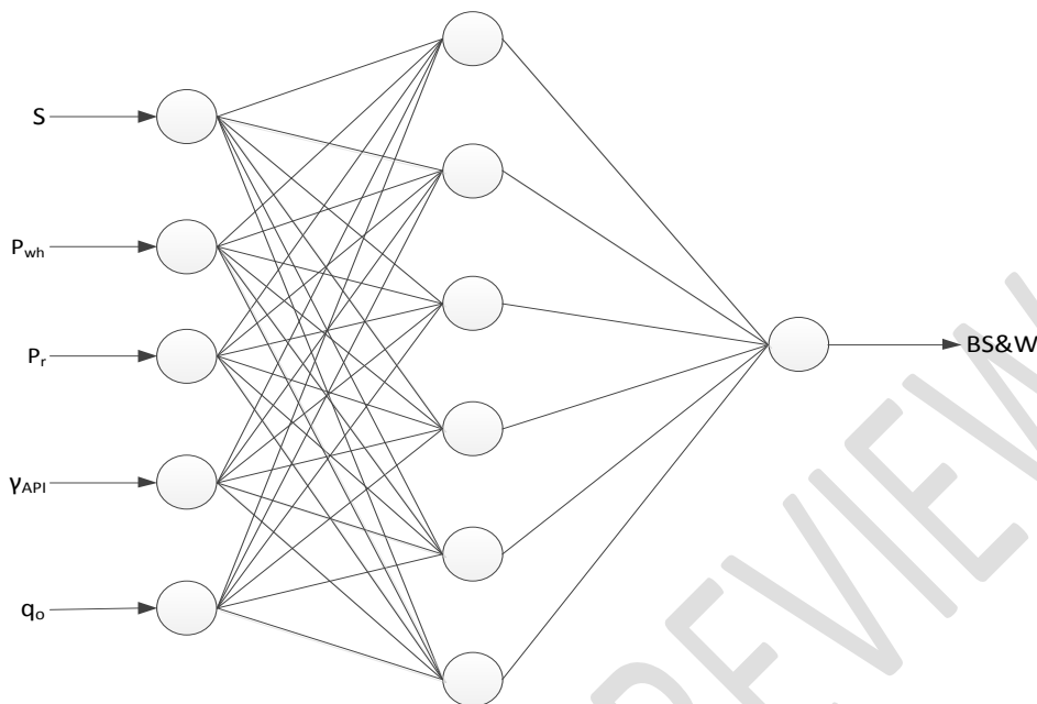
Figure 3: ANN Topology for BS&W Model
