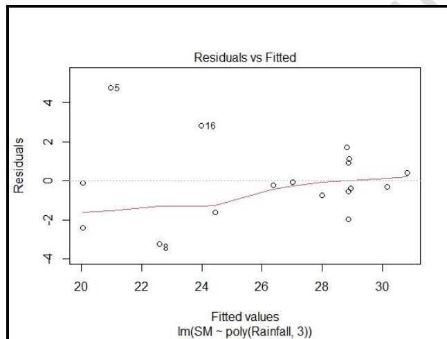
Fig. 9. The Residual vs. Fitted Plot between Rainfall and Soil Moisture
