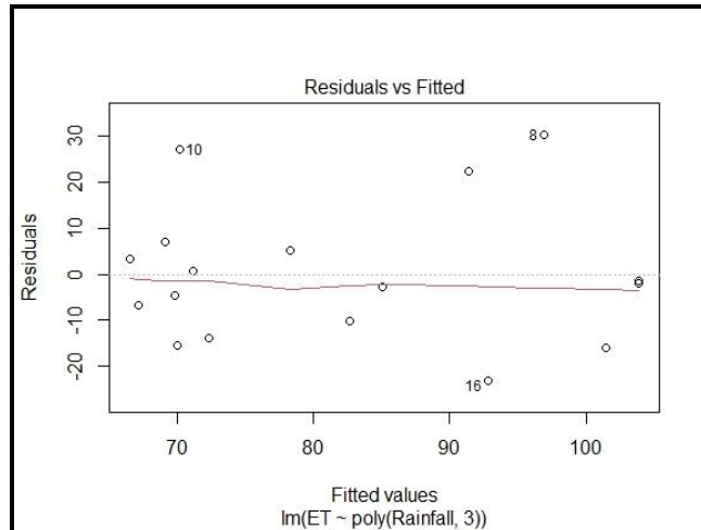
Fig. 11. The Residual vs. Fitted Plot between Rainfall and Evapotranspiration
