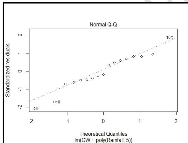
Fig. 14. The Normal Q-Q Plot between Rainfall and Depth to GW Table
