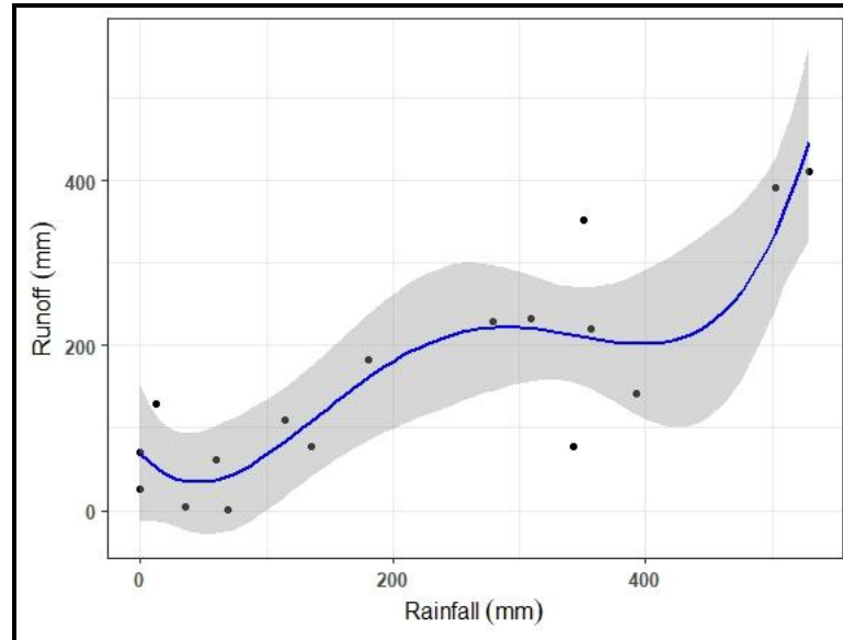
Fig. 4. Relation between Monthly Rainfall and Runoff
