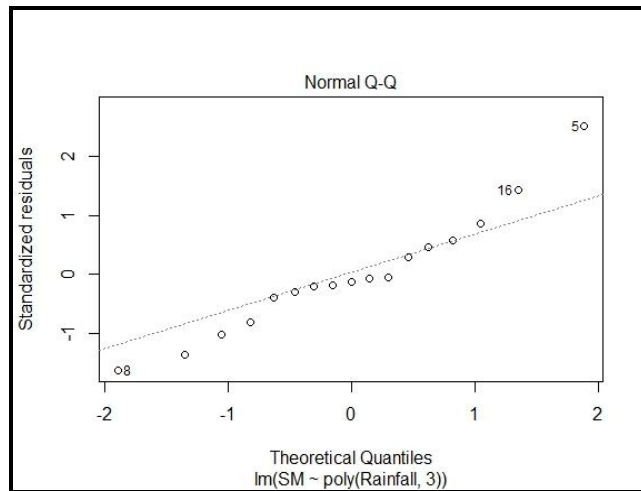
Fig. 13. The Normal Q-Q Plot between Rainfall and Soil Moisture
