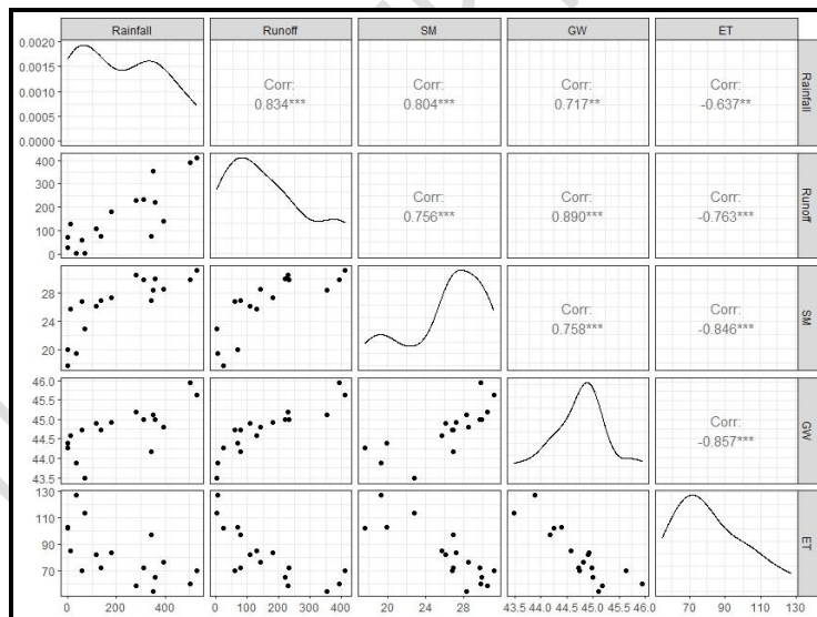
Fig. 2. Pearson's Correlation Coefficient for Perassannur Watershed
