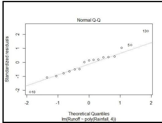
Fig. 11. The Normal Q-Q Plot between Rainfall and Runoff
