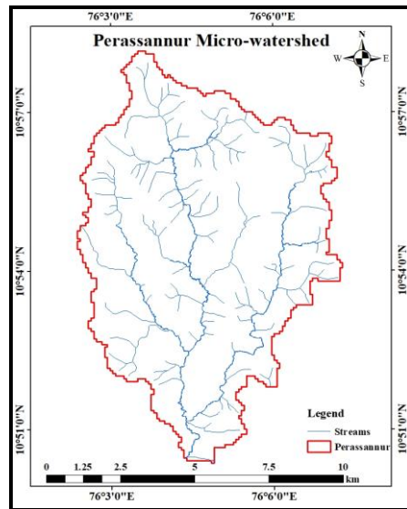
Fig.1. Perassannur Micro-watershed with Drainage Network
