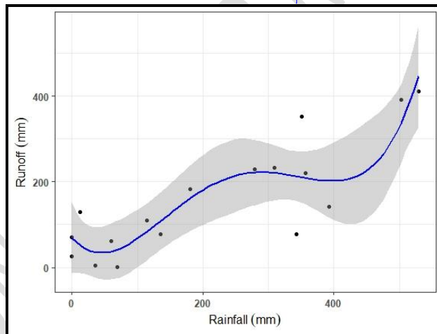
Fig. 3. Relation between Monthly Rainfall and Runoff
