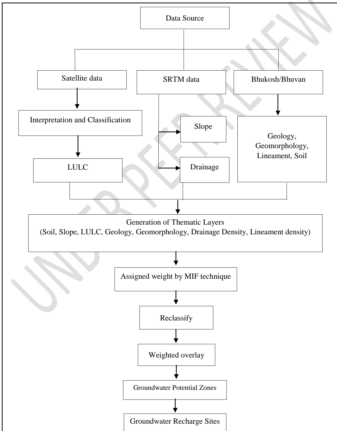
Fig 2. Procedure for identification of groundwater recharge sites
