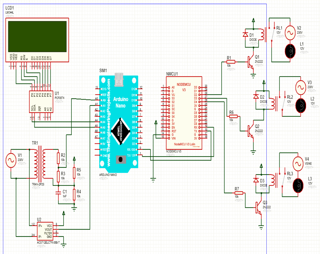
Fig. 8. Circuit Diagram of the Hardware Unit
