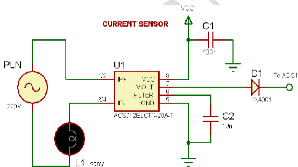
Fig.3. Current Sensing Unit
