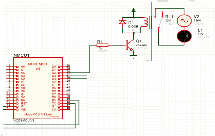
Fig. 7. Switching Unit
