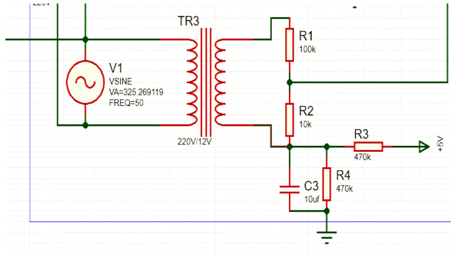
Fig.4. Voltage Sensing Unit
