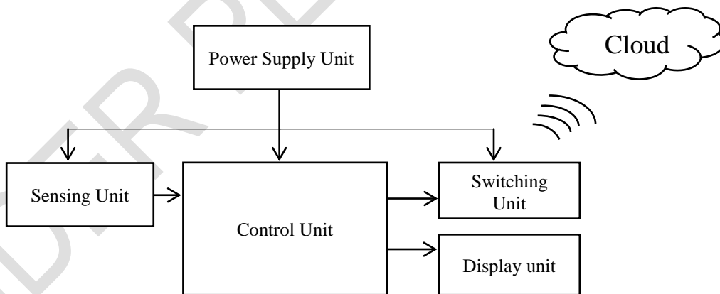
Fig.2. Block Diagram of the Hardware Development Unit
