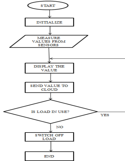
Fig. 11. Flowchart of the Developed Application
