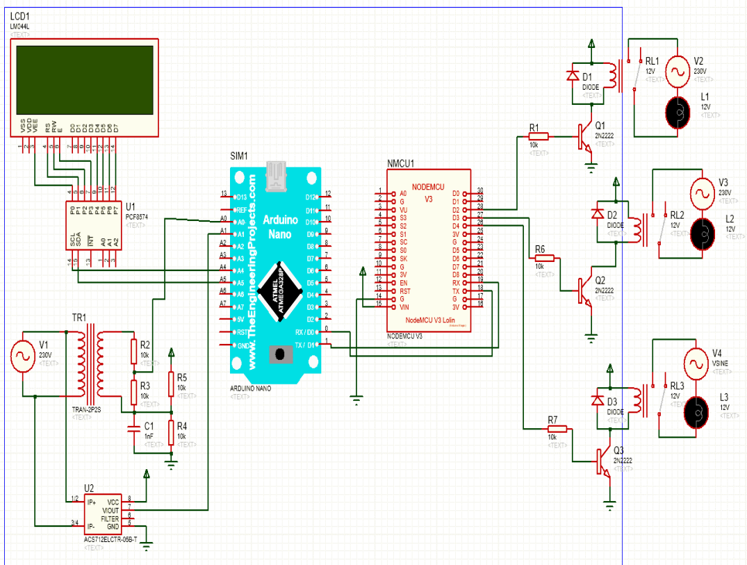
Fig.8. Circuit Diagram of the Hardware Unit
