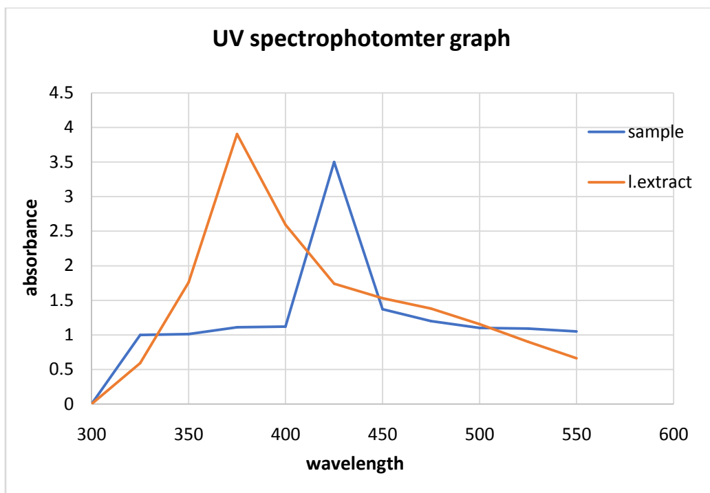
Fig.3UV-Spectrophotometric analysis of Silver nanoparticles
