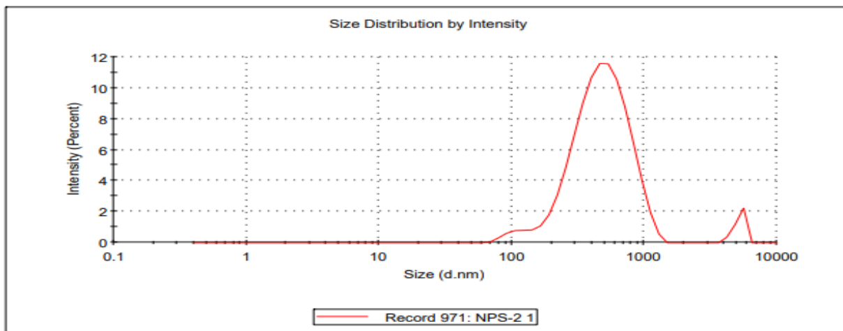
Fig.5DLS results of silver nanoparticles
