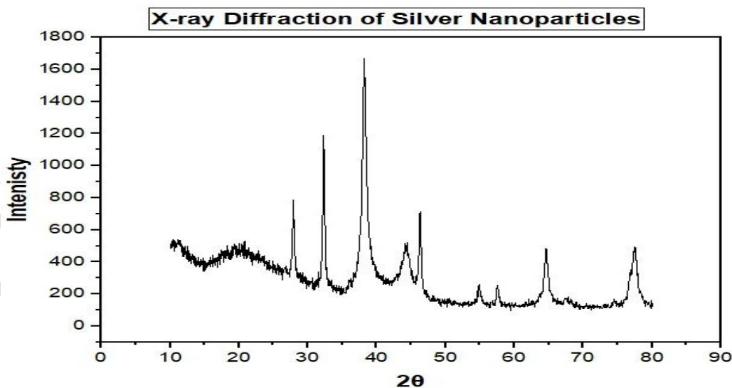
Fig.6Graph showing peaks of silver nanoparticle's
