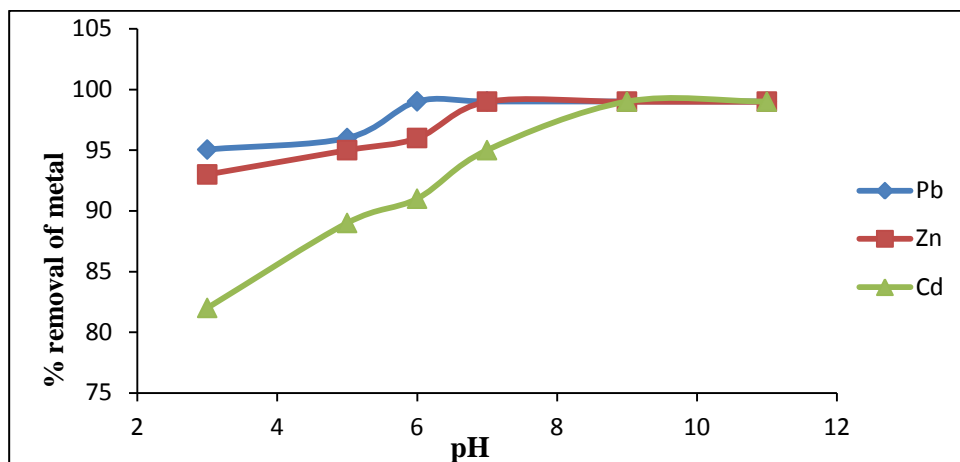
Fig. 10. Effect of pH on adsorption
