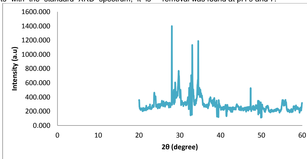
Fig. 9. XRD image of Bi-Mg bimetallic NP's
