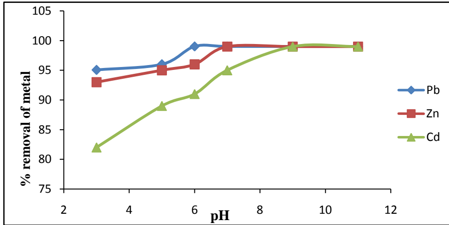
Fig. 10 Effect of pH on adsorption
