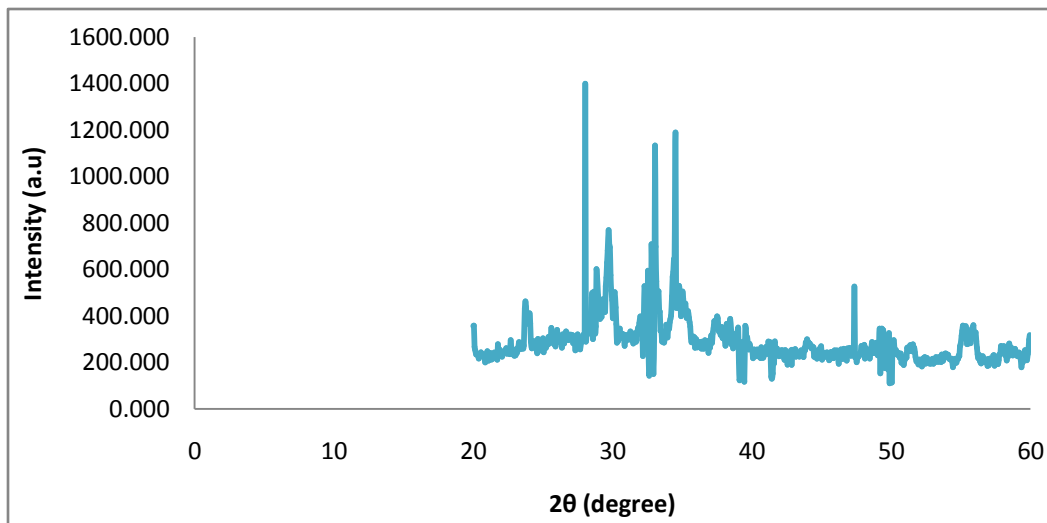
Fig. 9 XRD image of Bi-Mg bimetallic NP's
