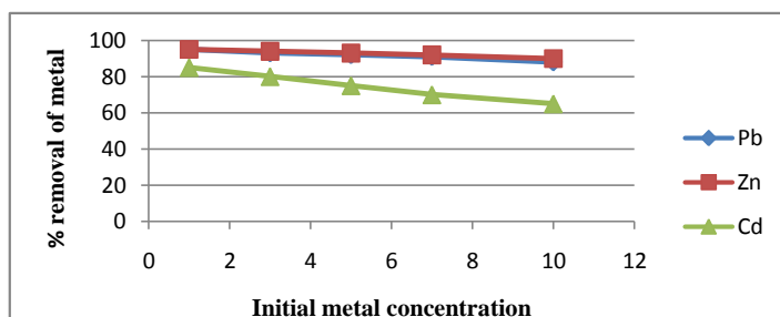
Figure- 12. Effect of initial metal concentrations
