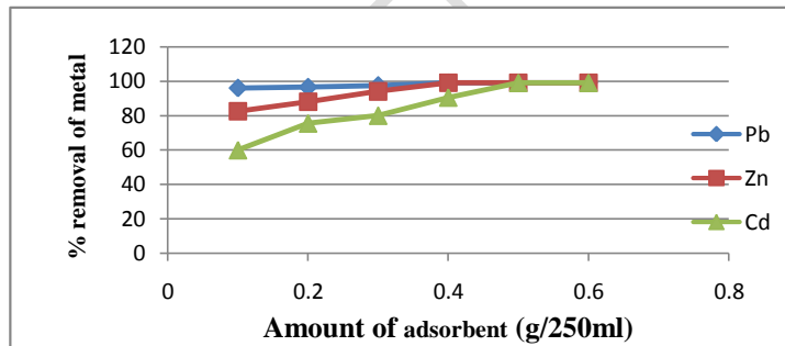
Figure 11. Effect of adsorbent dose on the removal of heavy metals
