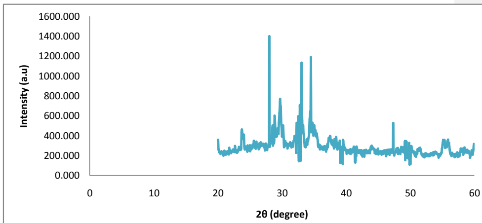
Figure- 9. XRD image of Bi-Mg bimetallic NP's
