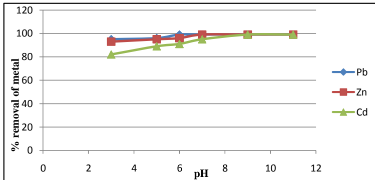
Figure 10. Effect of pH on adsorption
