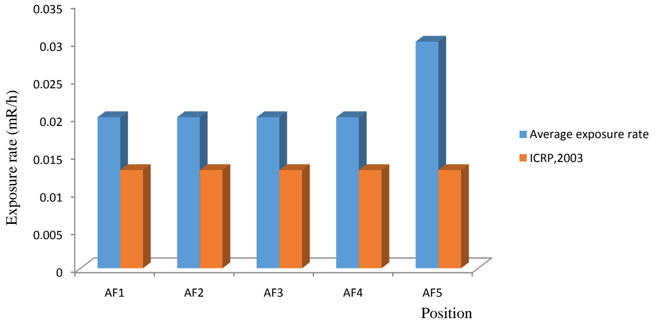
Fig 2: Comparison of Exposure rate in Soil with ICRP, 2003 Standard Value
