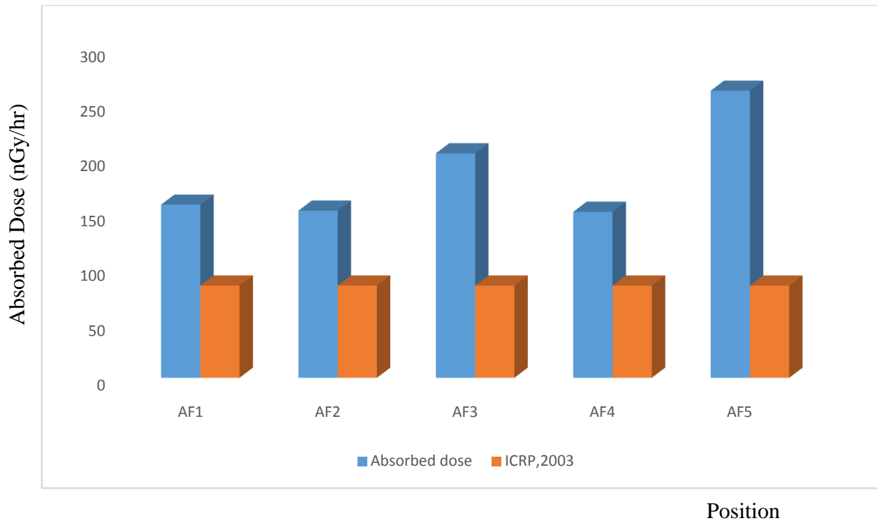
Fig 3: Comparison of Absorbed dose rate in Soil with ICRP, 2003 Standard Value
