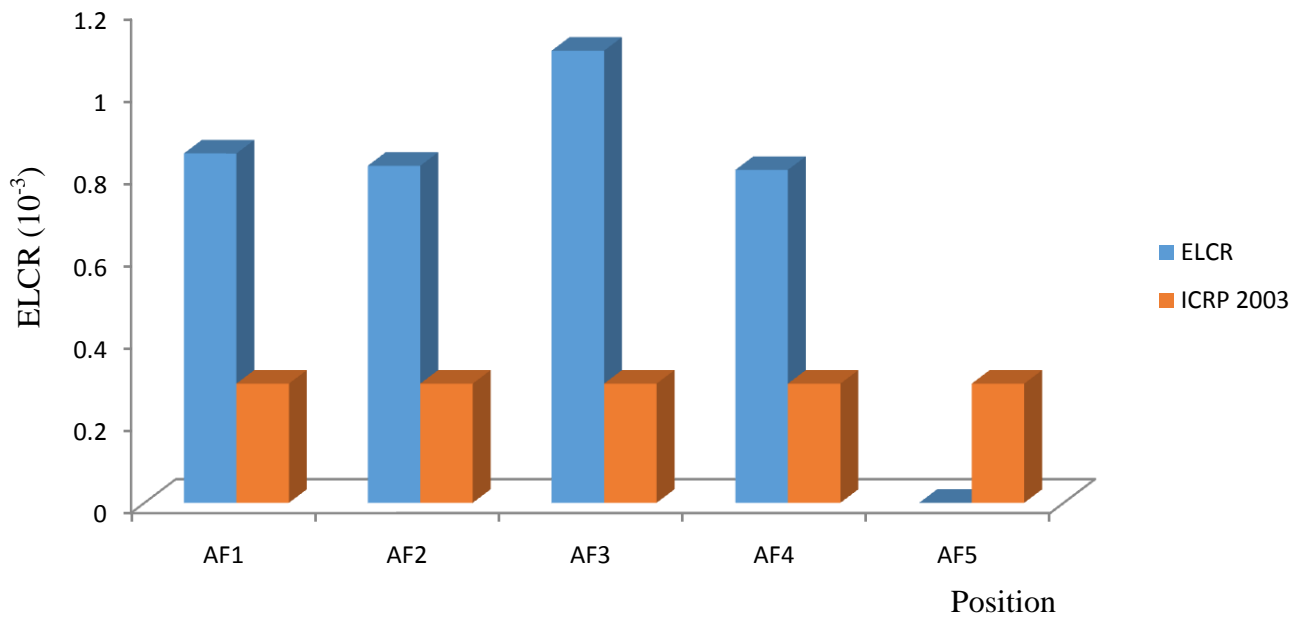
Fig 5: Comparison of Excess Life Cancer Risk in Soil with ICRP, 2003 Standard Value
