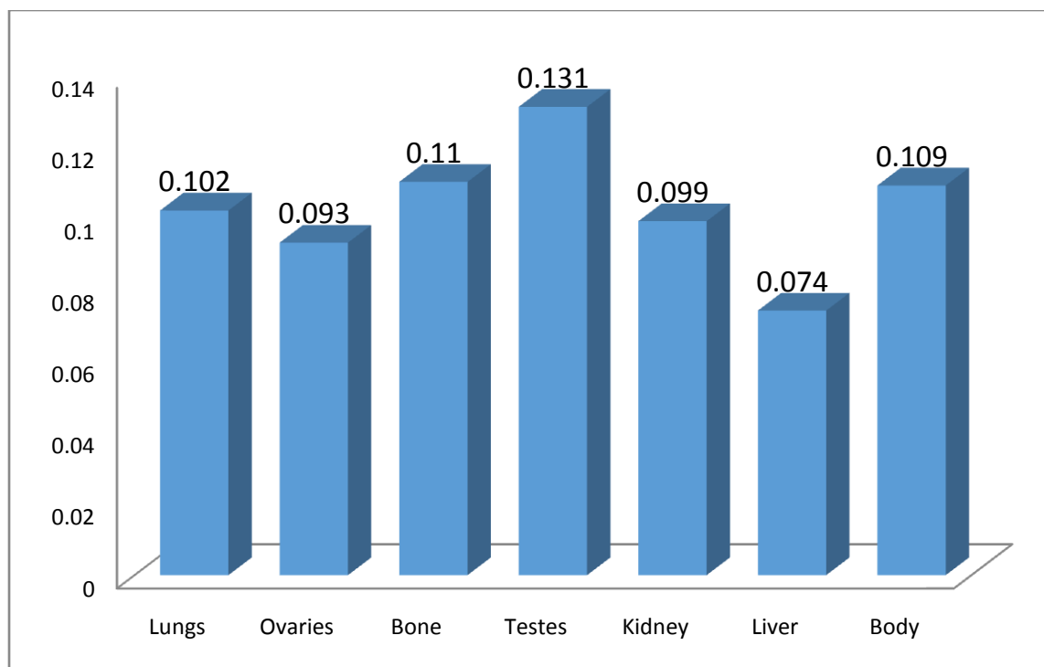
Fig 6: Effective Dose Rate (in mSv/y) to Different Organs/Tissues
