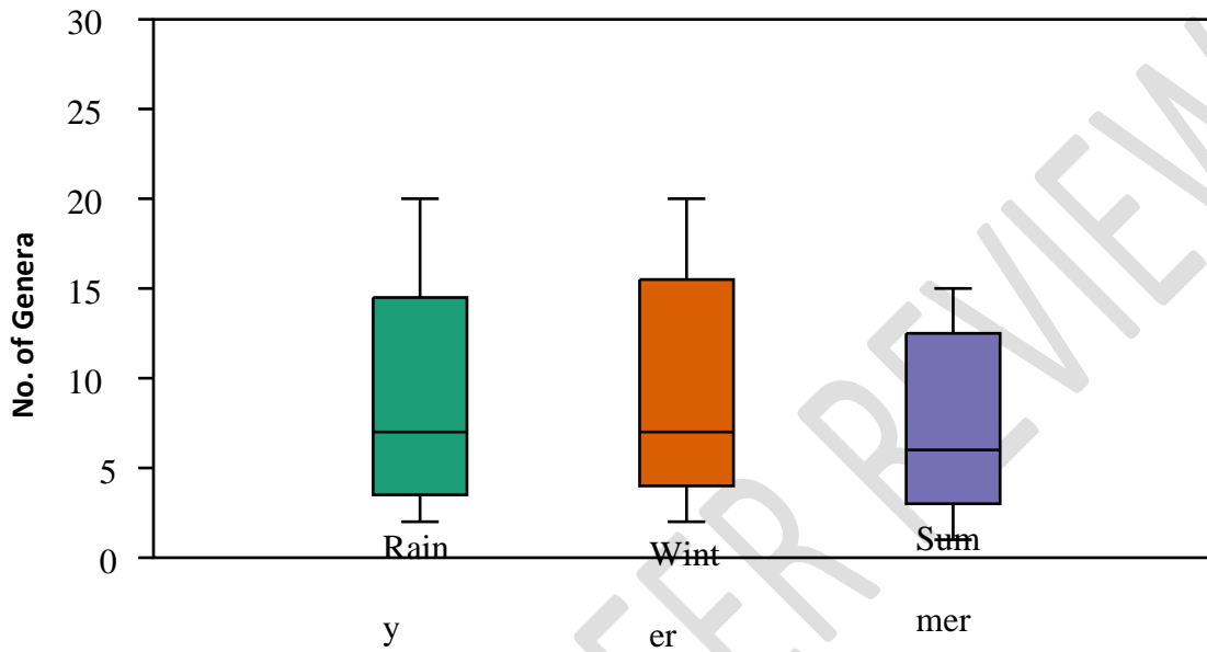
Fig. 3. Seasonal distribution of various Genera
