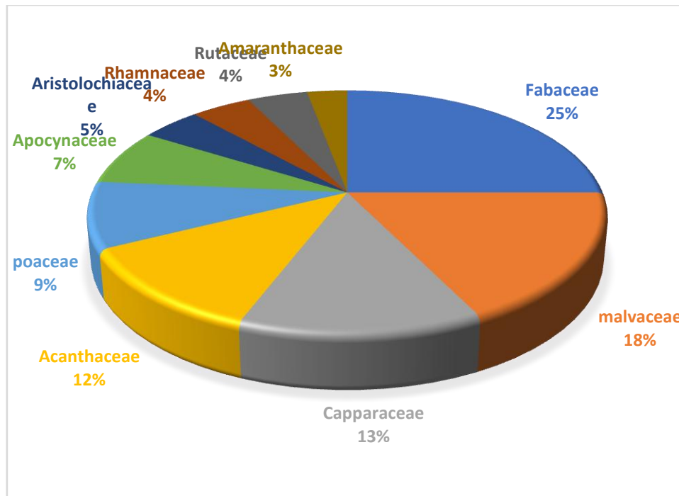
Fig. 1. Top host plant families
