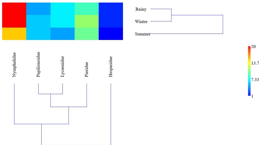
Fig. 4. Hierarchical cluster analysis of Bray-Curti's similarity index
