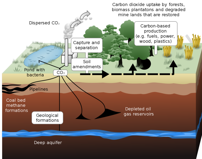
Image 1: Carbon sequestration
