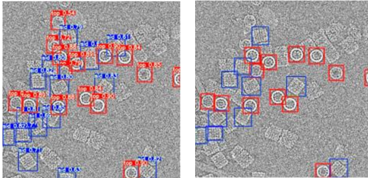
Fig. 3. The image output with the confidence associate to each detection (left) can be used to tune the inference and reduce the number of false positives, using a higher confidence threshold, in the case 0.75 (right)
