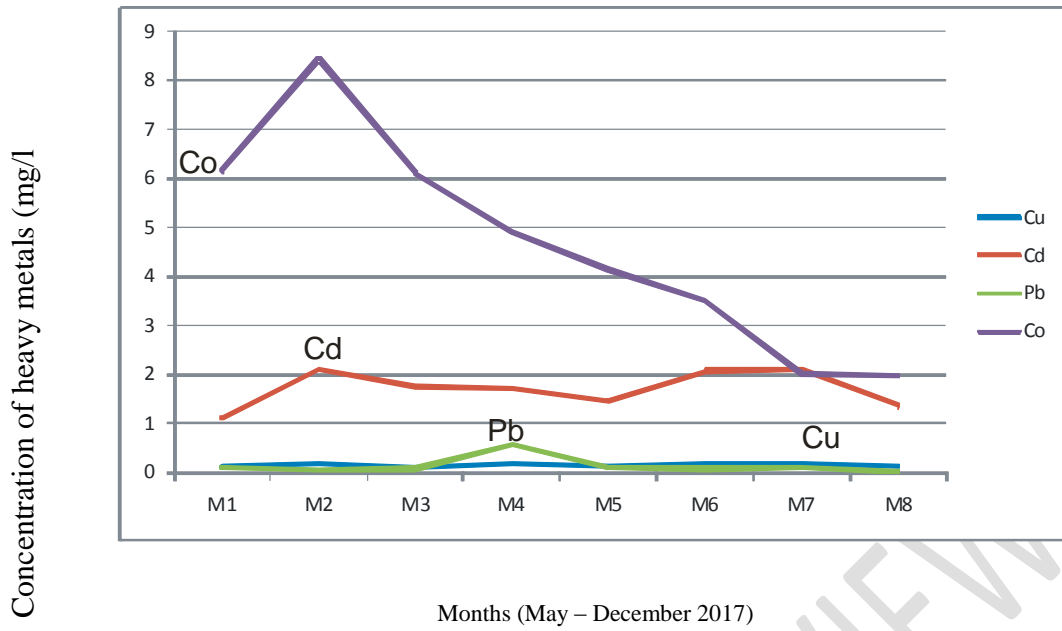
Figure 4. The trend of accumulation of heavy metals at sampling point 4 in the Wulmi River
