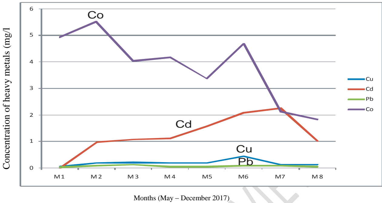
Figure 2. The trend of accumulation of heavy metals at sampling point 2 in the Wulmi River
