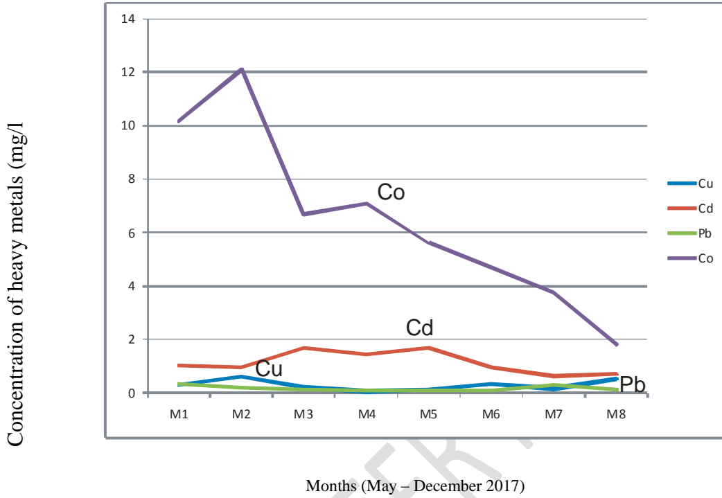
Figure 1. The trend of accumulation of heavy metals at sampling point 1 in the Wulmi River
