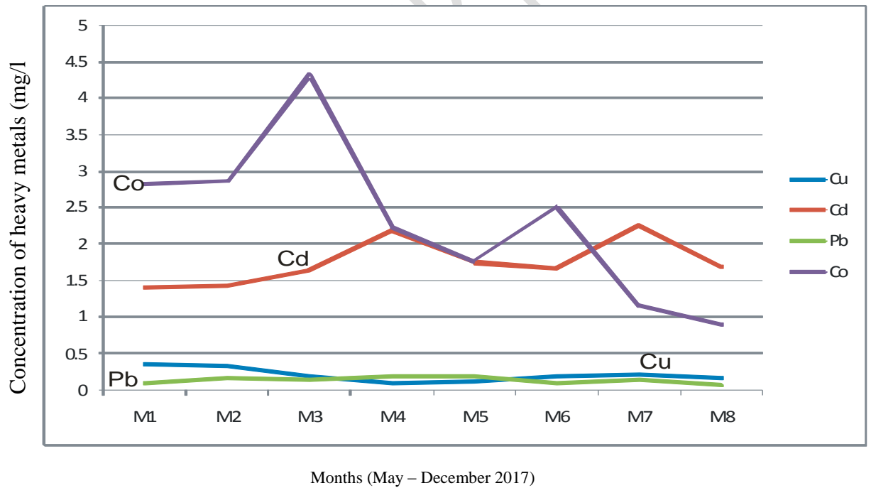
Figure 3. Trend of accumulation of heavy metals at sampling point 3 in Wulmi River
