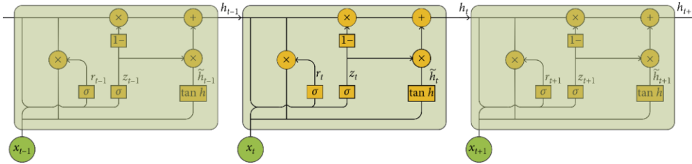
Figure 2: GRU Architecture
