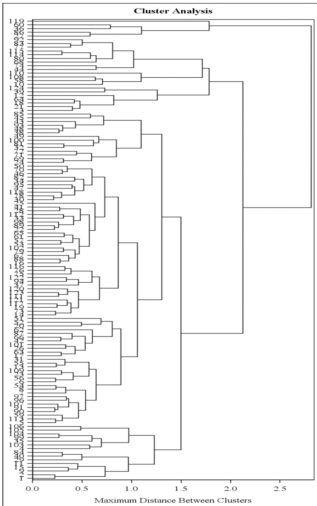
Fig.1 Cluster diagram of 124 muskmelon genotypes developed through Tocher's method using D^2 statistics.
