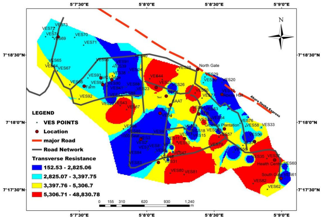
Fig. 7: Transverse resistance map of the area
