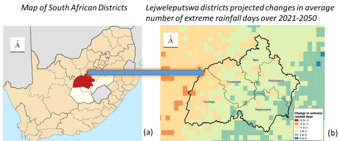
Figure 1: map showing the South African districts, Lejweleputswa district, its local municipalities indicating change in extreme rainfall days (CSIR, 2019).
