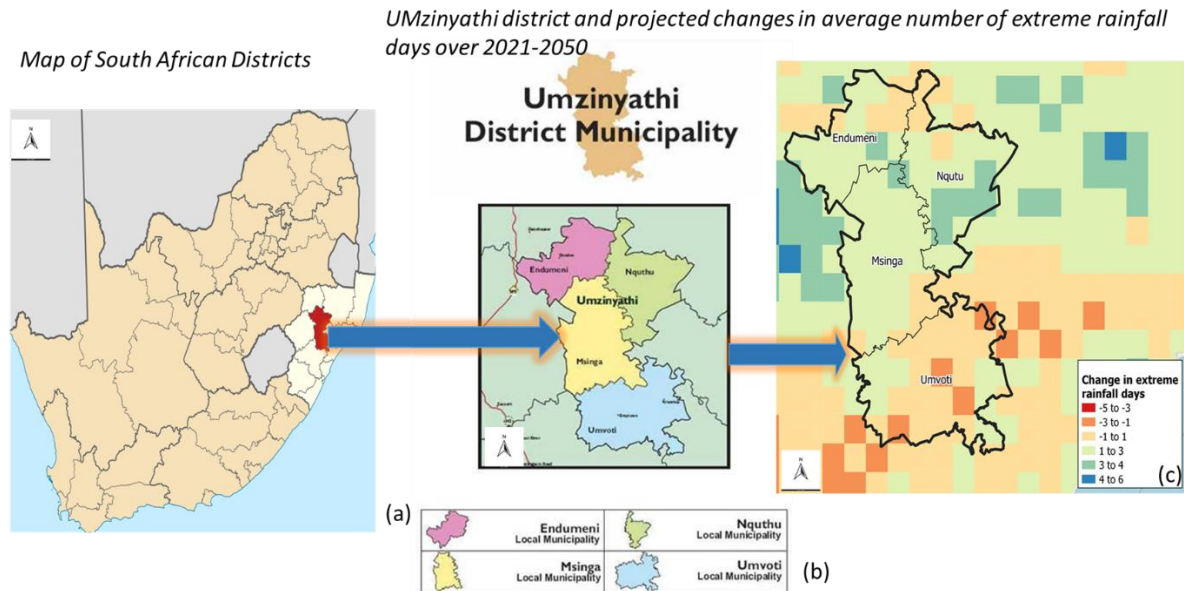
Figure 2: map showing the South African districts, UMzinyathi district, its local municipalities indicating change in extreme rainfall days (CSIR, 2019).
