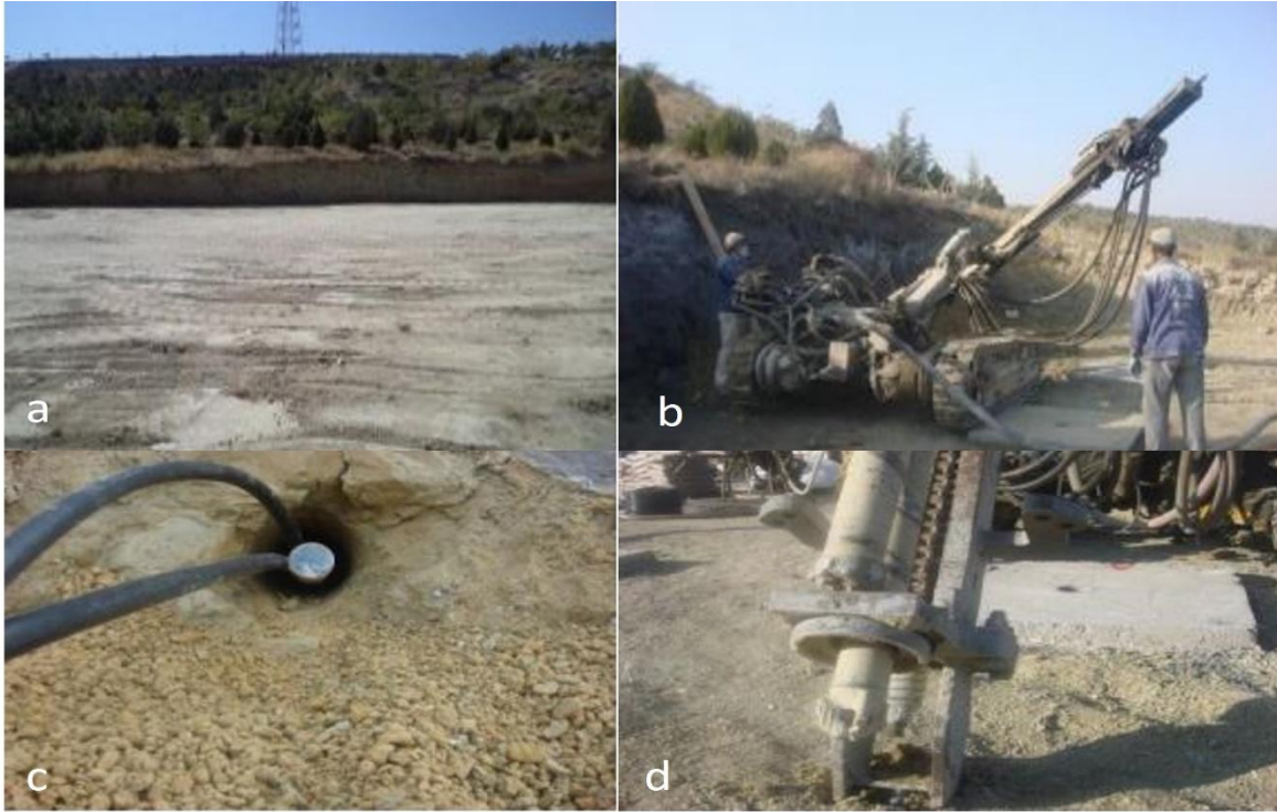
Figure 2. Site preparation and the method of implementing a reinforced concrete foundation for pile installation. (a) Site leveling and preparation. (b) The excavation machine used in the project. (c) Excavation, placement of reinforcement, and installation of grout injection pipes. (d) The method of using rotary drilling in the project.
