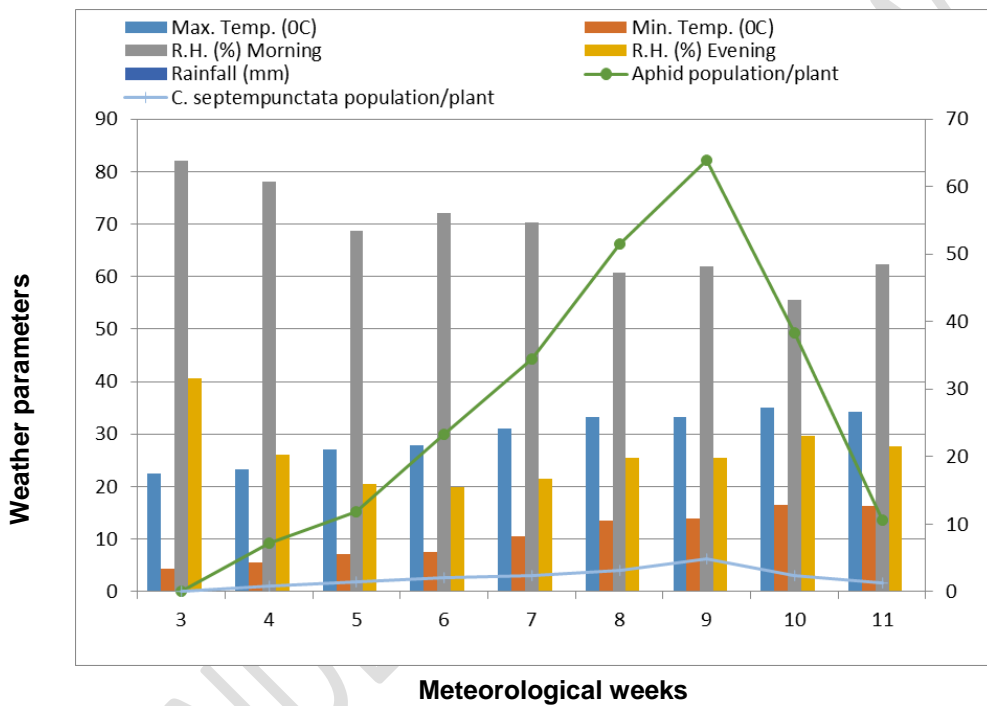
Fig. 1 Population dynamics of coriander aphid and their correlation with biotic and abiotic factors during Rabi , 2020-
