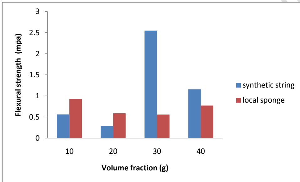
Figure 3: Effect of fibre on Flexural strength.
