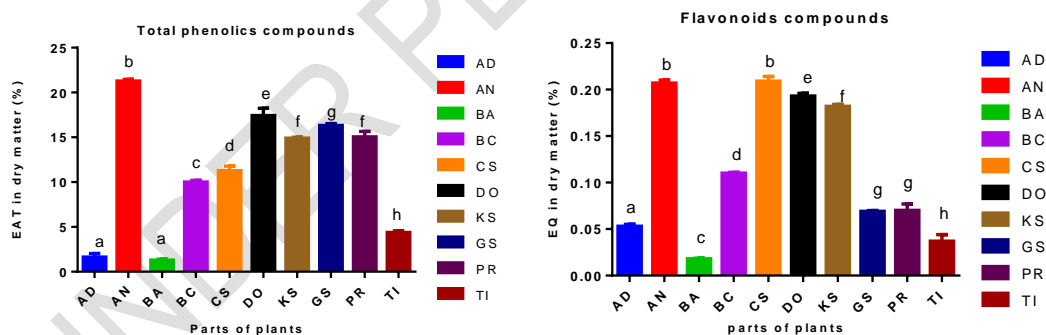
Figure 1 : Total phenolic and flavonoid content of extracts from different plants
