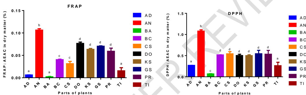
Figure 2: Antioxidant activity by the FRAP and DPPH method of extracts from different plants
