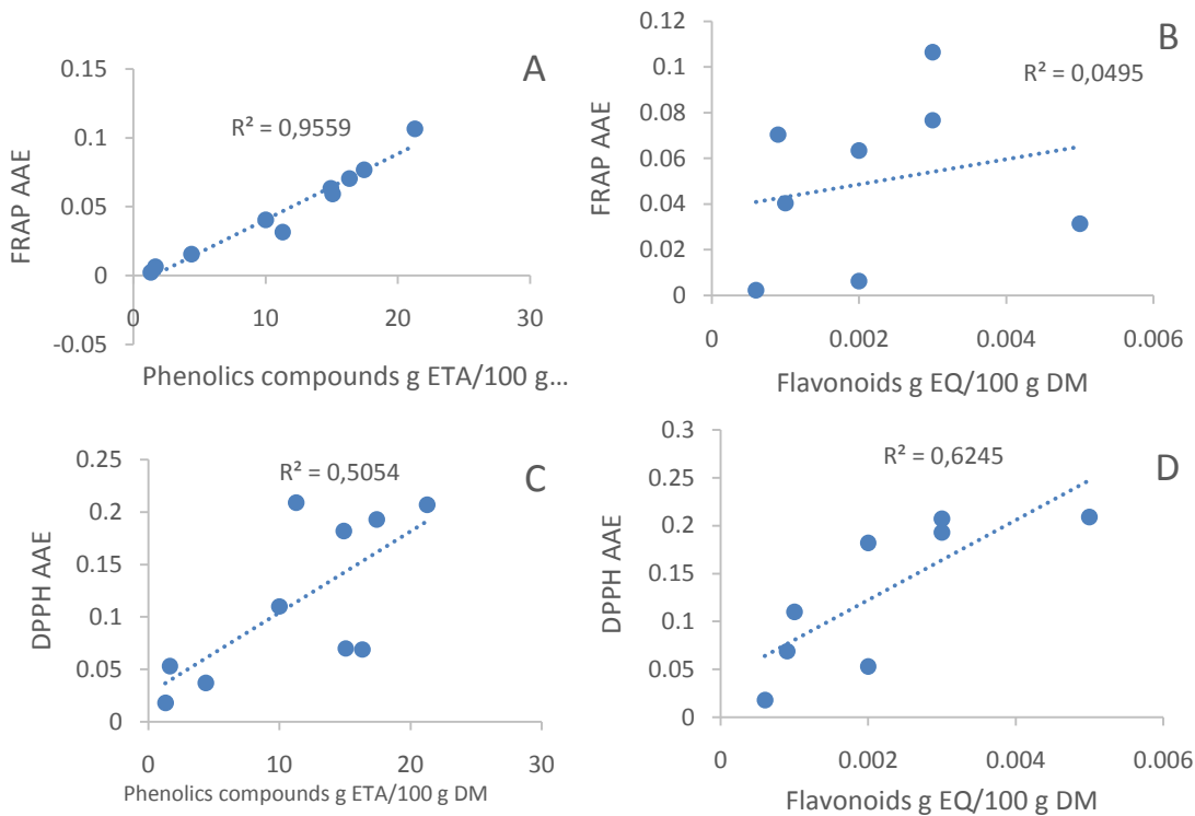
Figure 3 : Correlation between FRAP and the total phenolics content (A) and between FRAP and total flavonoid content (B); Correlation between DPPH and the total phenolics content (C) and between DPPH f and total flavonoid content (D)
