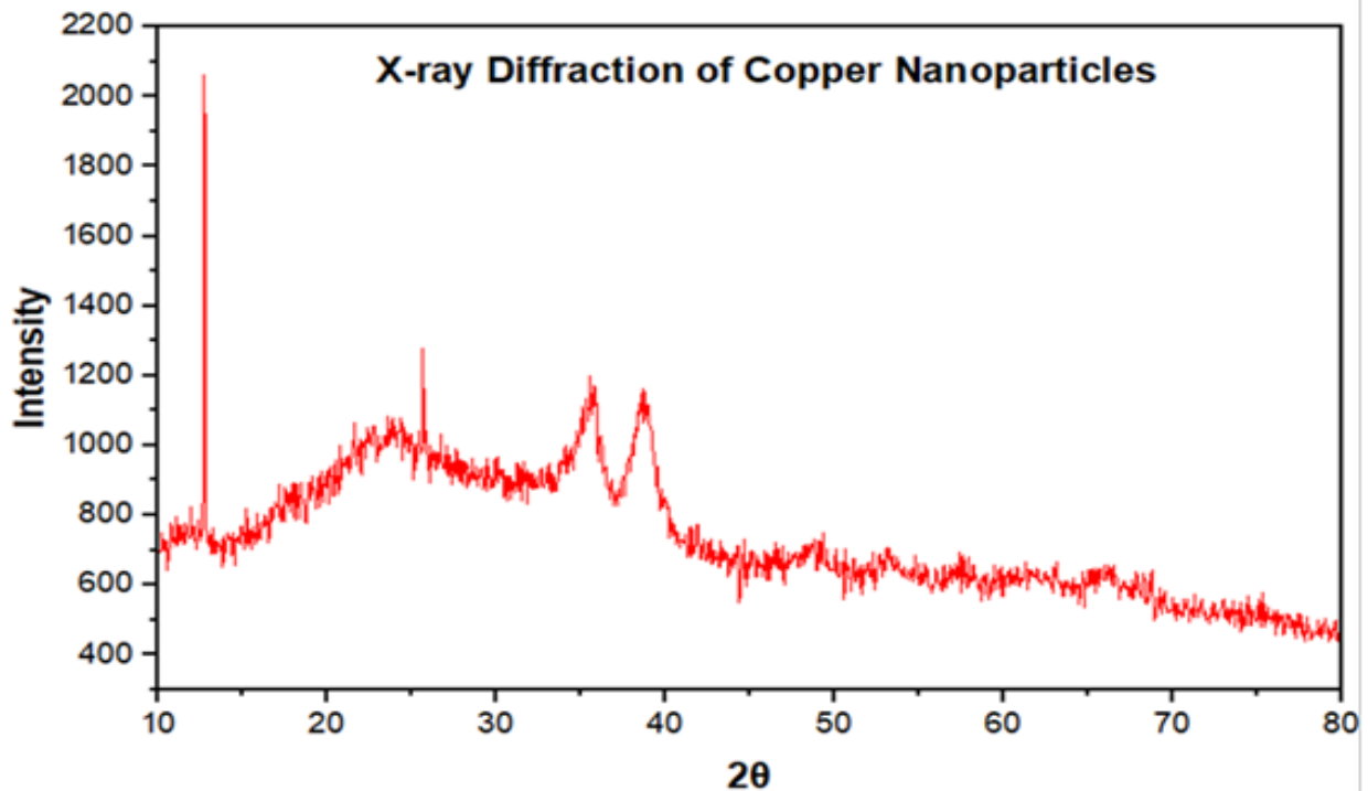
Fig 10. XRD graphs of copper nanoparticles
