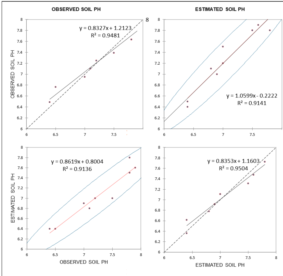
Figure 2.a: R2 results for remote sensing-based Soil pH correlations with sorghum field data
