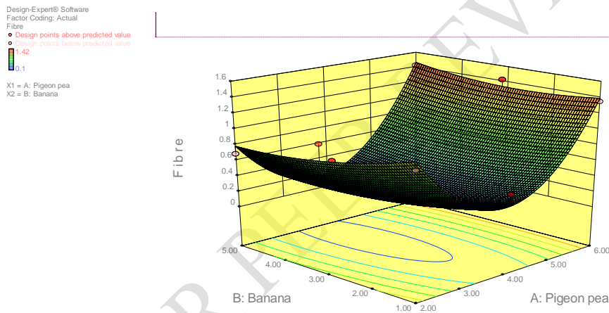
Fig.3: Surface plot for the fibre content of the enriched rice-based breakfast cereal
