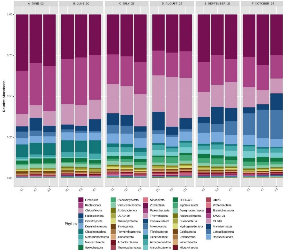
Figure 5. Bar plot representing the relative abundance of the bacterial and archaeal phyla in anaerobic sludge.
