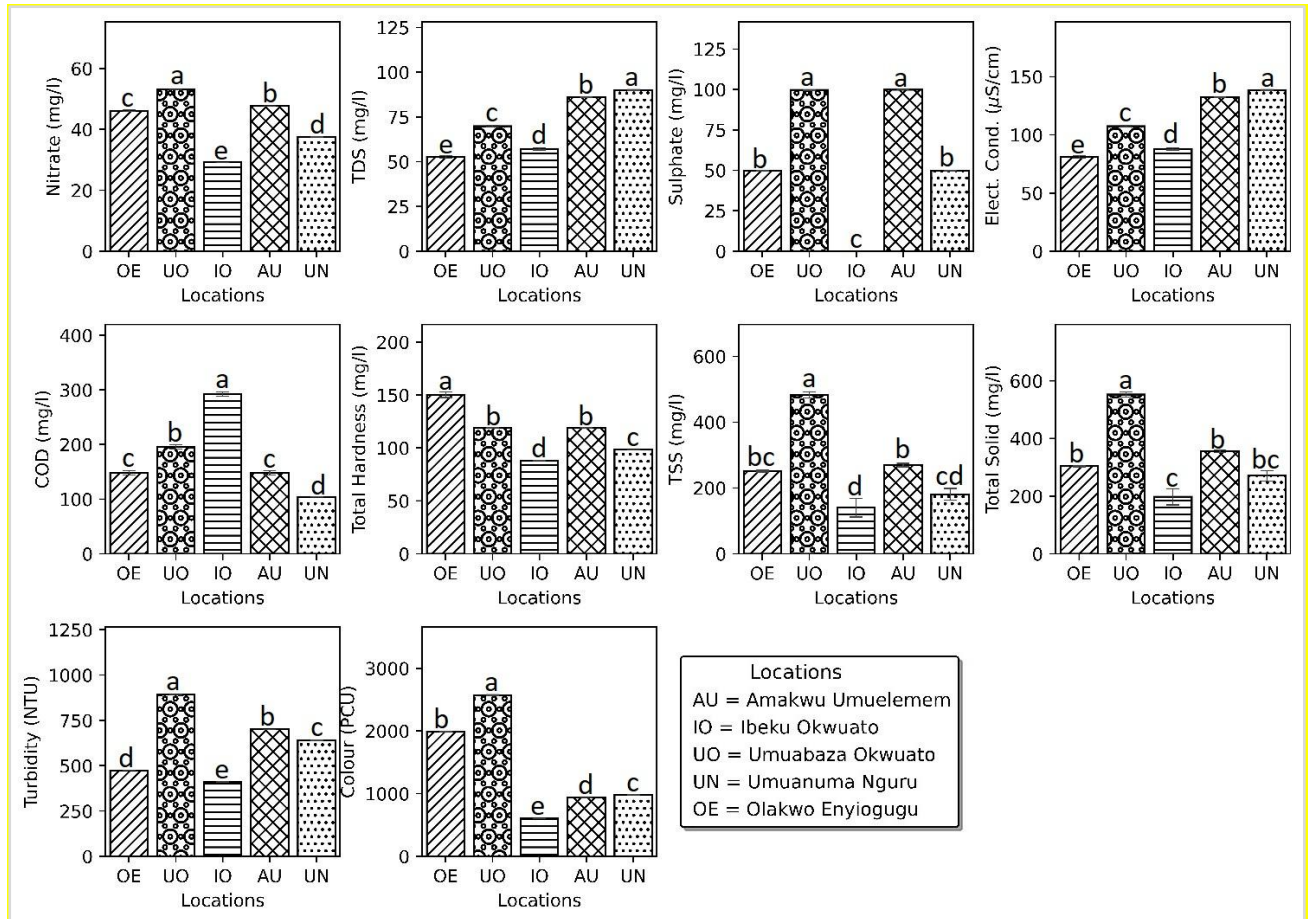
Figure 2b: Barplots showing test of significance of the various physiochemical parameter: NO 3 , TDS, SO 4 , EC, COD, TH, TSS, TS, Tur. & Colour
