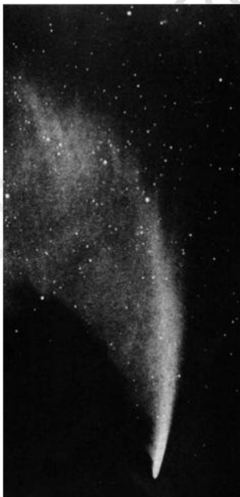
Figure 3. Comet Halley observed in 1910.
