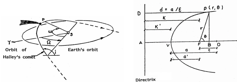
Figure 7. orbital elements of Halley comet. (NEVES & ARGUELLO, 1986)
