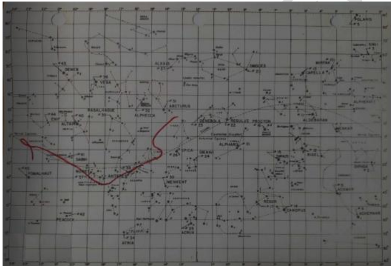
Figure 21. Neowise: calculated trajectory by MRTE.
