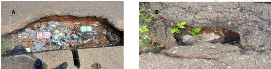
Figure 2. (a) Sinkhole at Awka site 1 (b) Soil pipe at Awka site 2
